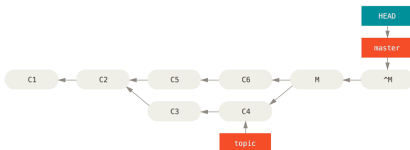
FIGURE 7-22 History after git revert -m 1
