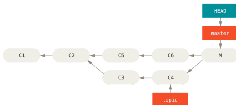
FIGURE 7-20 Accidental merge commit
