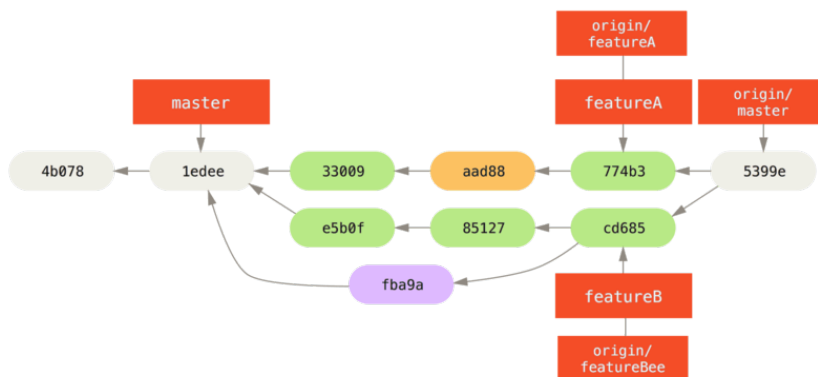
FIGURE 5-15 Jessica's history after merging both her topic branches.
