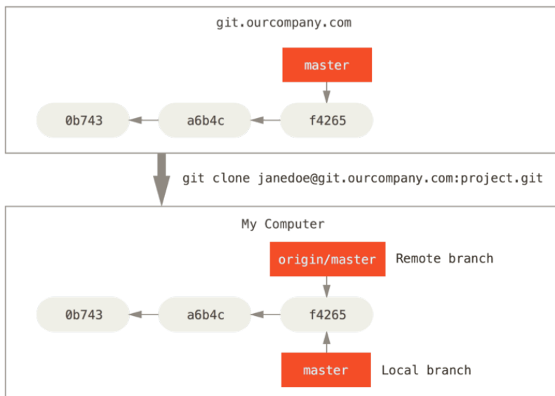
FIGURE 3-22 Server and local repositories after cloning
