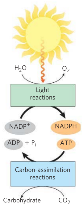
FIGURE 19-46 The light reactions of photosynthesis generate energy-rich NADPH and ATP at the expense of solar energy. NADPH and ATP are used in the carbon-assimilation reactions, which occur in light or darkness, to reduce CO 2 to form trioses and more complex compounds (such as glucose) derived from trioses.
