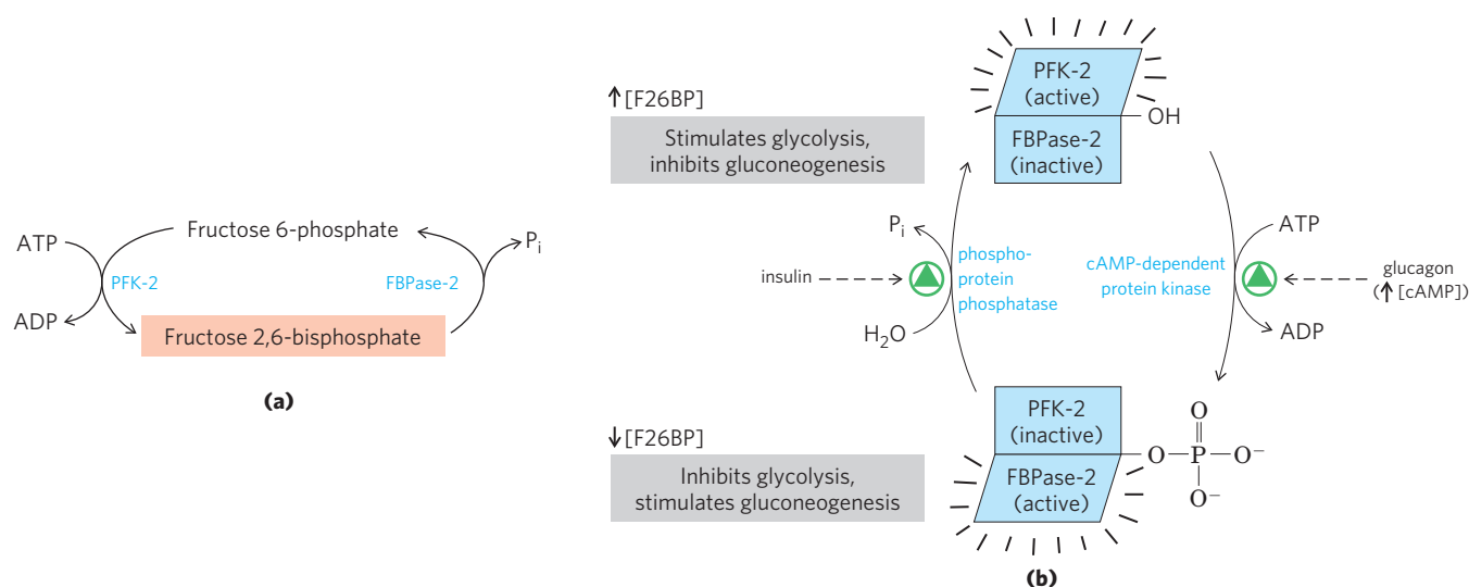
FIGURE 15-19 Regulation of fructose 2,6-bisphosphate level. (a) The cellular concentration of the regulator fructose 2,6-bisphosphate (F26BP) is determined by the rates of its synthesis by phosphofruktokinase-2 (PFK-2) and its breakdown by fructose 2,6-bisphosphatase (FBPase-2). (b) Both enzyme activities are part of the same polypeptide chain, and they are reciprocally regulated by insulin and glucagon.
