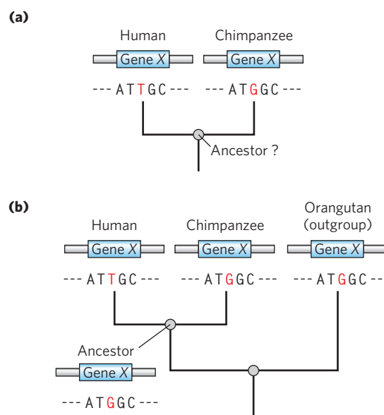
FIGURE 9-32 Determination of sequence alterations unique to one ancestral line. (a) Sequences from the same hypothetical gene in humans and chimpanzees are compared. The sequence of this gene in their last common ancestor is unknown. (b) The orangutan genome is used as an outgroup. The sequence of the orangutan gene is identical to the chimpanzee gene. This means that the mutation causing the difference between humans and chimpanzees almost certainly occurred in the line leading to modern humans, and the common ancestor of humans and chimpanzees (and orangutans) had the sequence now found in chimpanzees.
