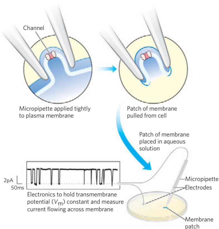
FIGURE 11–46 Electrical measurements of ion-channel function.
