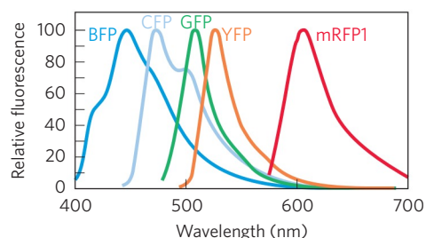
FIGURE 4 Emission spectra of GFP variants.
