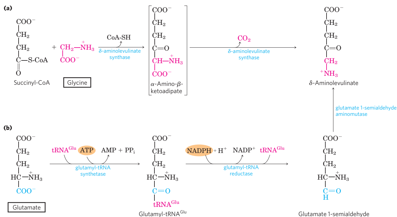
FIGURE 22-25 Biosynthesis of \delta -aminolevulinic acid. (a) In most animals, including mammals, \delta -aminolevulinic acid is synthesized from glycine and succinyl-CoA. The atoms furnished by glycine are shown in red. (b) In bacteria and plants, the precursor of \delta -aminolevulinic acid is glutamate.
