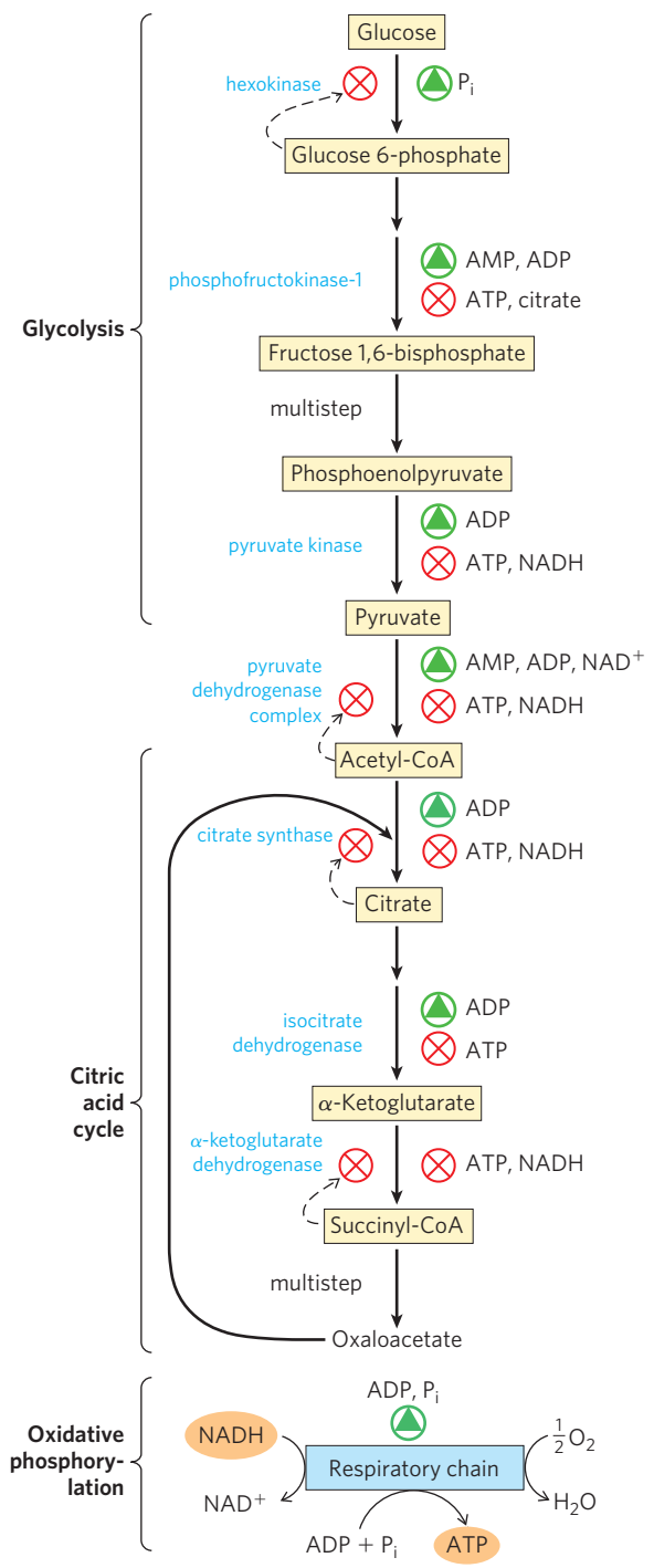
FIGURE 19-35 Regulation of the ATP-producing pathways. This diagram shows the interlocking regulation of glycolysis, pyruvate oxidation, the citric acid cycle, and oxidative phosphorylation by the relative concentrations of ATP, ADP, and AMP, and by NADH. High [ATP] (or low [ADP] and [AMP]) produces low rates of glycolysis, pyruvate oxidation, acetate oxidation via the citric acid cycle, and oxidative phosphorylation. All four pathways are accelerated when the use of ATP and the formation of ADP, AMP, and P_i increase. The interlocking of glycolysis and the citric acid cycle by citrate, which inhibits glycolysis, supplements the action of the adenine nucleotide system. In addition, increased levels of NADH and acetyl-CoA also inhibit the oxidation of pyruvate to acetyl-CoA, and a high [NADH]/[NAD^+] ratio inhibits the dehydrogenase reactions of the citric acid cycle (see Fig. 16-19).
