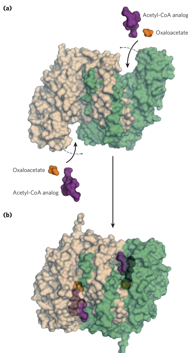
FIGURE 16-8 Structure of citrate synthase. The flexible domain of each subunit undergoes a large conformational change on binding oxaloacetate, creating a binding site for acetyl-CoA. (a) Open form of the enzyme alone (PDB ID 5CSC); (b) closed form with bound oxaloacetate and a stable analog of acetyl-CoA (carboxymethyl-CoA) (derived from PDB ID 5CTS). In these representations one subunit is colored tan and one green.
