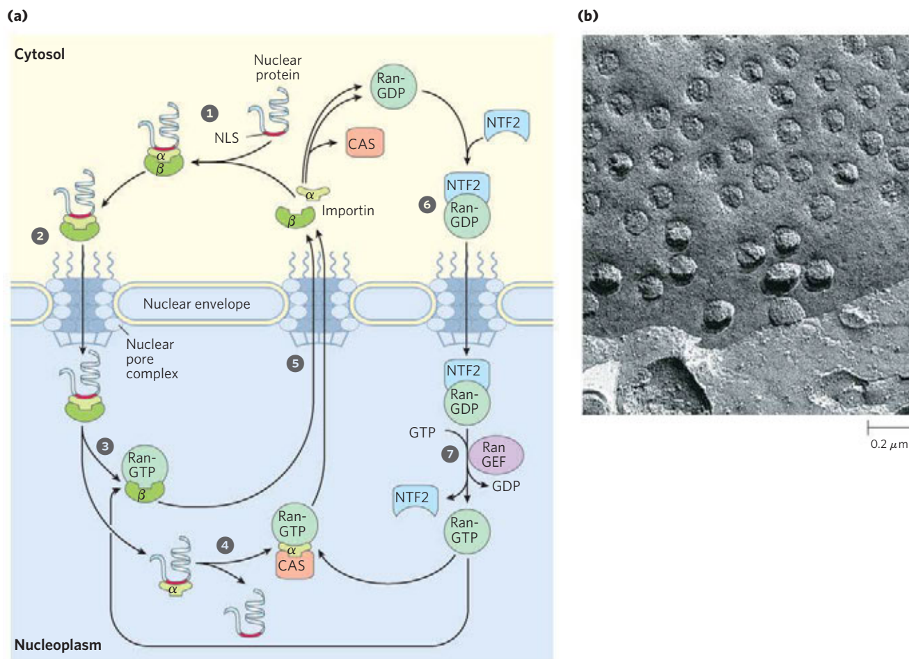
FIGURE 27–42 Targeting of nuclear proteins. (a) 1 A protein with an appropriate nuclear localization signal (NLS) is bound by a complex of importin \alpha and \beta . 2 The resulting complex binds to a nuclear pore and translocates. 3 Inside the nucleus, dissociation of importin \beta is promoted by the binding of Ran-GTP. 4 Importin \alpha binds to Ran-GTP and CAS (cellular apoptosis susceptibility protein), releasing the nuclear protein. 5 Importin \alpha and \beta and CAS are transported out of the nucleus and recycled. They are released in the cytosol when Ran hydrolyzes its bound GTP.
