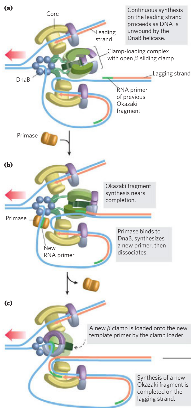
FIGURE 25-13 DNA synthesis on the leading and lagging strands.
