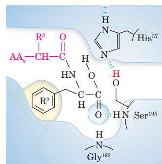
Enzyme-product 2 complex
