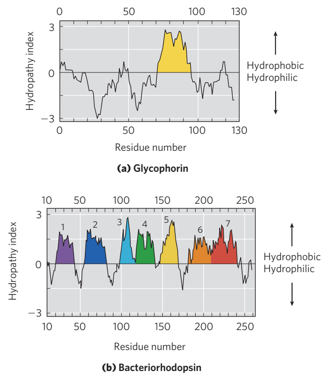
FIGURE 11-12 Hydropathy plots. Average hydropathy index (see Table 3-1) is plotted against residue number for two integral membrane proteins. The hydropathy index for each amino acid residue in a sequence of defined length, or “window,” is used to calculate the average hydropathy for that window. The horizontal axis shows the residue number in the middle of the window. (a) Glycophorin from human erythrocytes has a single hydrophobic sequence between residues 75 and 93 (yellow); compare this with Figure 11-8. (b) Bacteriorhodopsin, known from independent physical studies to have seven transmembrane helices (see Fig. 11-10), has seven hydrophobic regions. Note, however, that the hydropathy plot is ambiguous in the region of segments 6 and 7. X-ray crystallography has confirmed that this region has two transmembrane segments.
