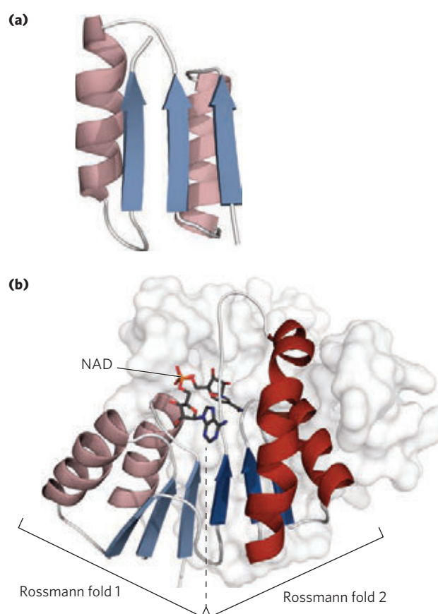
FIGURE 13–25 The Rossmann fold. This structural motif is found in the NAD -binding site of many dehydrogenases. (a) It consists of a pair of structurally similar motifs (only one of which is shown here), each having three parallel \beta sheets and two \alpha helices ( \beta - \alpha - \beta - \alpha - \beta ). (b) The nucleotide-binding domain of the enzyme lactate dehydrogenase (derived from PDB ID 3LDH) with NAD (ball-and-stick structure) bound in an extended conformation through hydrogen bonds and salt bridges to the paired \beta - \alpha - \beta - \alpha - \beta motifs of the Rossmann fold (shades of red and blue).
