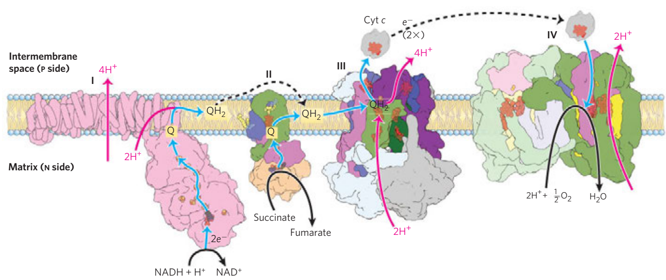
FIGURE 19-16 Summary of the flow of electrons and protons through the four complexes of the respiratory chain. Electrons reach Q through Complexes I and II. The reduced Q (QH 2 ) serves as a mobile carrier of electrons and protons. It passes electrons to Complex III, which passes them to another mobile connecting link, cytochrome c. Complex IV then transfers electrons from reduced cytochrome c to O 2 . Electron flow through Complexes I, III, and IV is accompanied by
