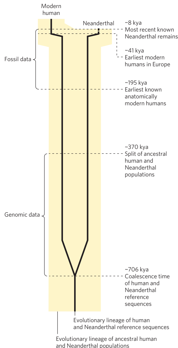
FIGURE 2 This timeline shows the divergence of human and Neanderthal genome sequences (black lines) and of ancestral human and Neanderthal populations (yellow screen). Genomic data provide evidence for some intermingling of the populations up to about 45,000 years ago. Key events in human evolution are noted.
