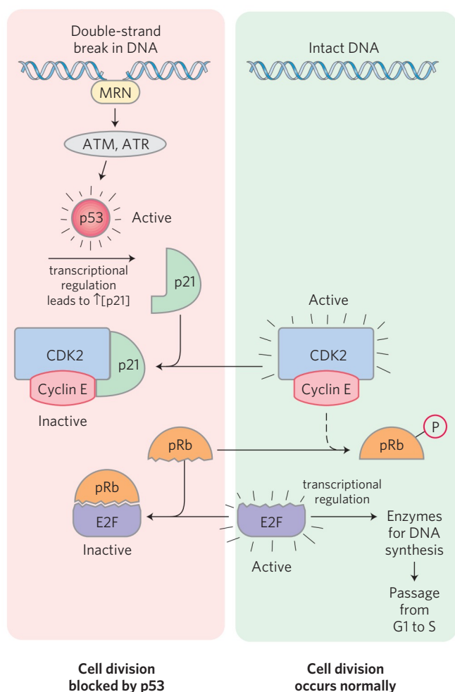
FIGURE 12–49 Regulation of passage from G1 to S by phosphorylation of pRb. Transcription factor E2F promotes transcription of genes for certain enzymes essential to DNA synthesis. The retinoblastoma protein, pRb, can bind E2F (lower left), inactivating it and preventing transcription of these genes. Phosphorylation of pRb by CDK2 prevents it from binding and inactivating E2F, and the genes are transcribed, allowing cell division. Damage to the cell's DNA (upper left) triggers a series of events that inactivate CDK2, blocking cell division. When the protein MRN detects damage to the DNA, it activates two protein kinases, ATM and ATR, and they phosphorylate and activate the transcription factor p53. Active p53 promotes the synthesis of another protein, p21, an inhibitor of CDK2. Inhibition of CDK2 stops the phosphorylation of pRb, which therefore continues to bind and inhibit E2F. With E2F inactivated, genes essential to cell division are not transcribed and cell division is blocked. When DNA has been repaired, this inhibition is released, and the cell divides.
