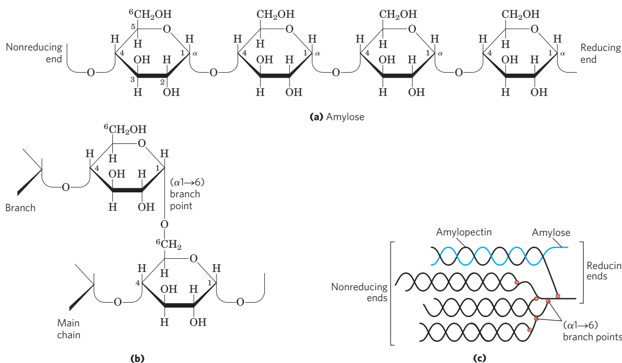
FIGURE 7-13 Glycogen and starch. (a) A short segment of amylose, a linear polymer of D-glucose residues in (\alpha 1 \rightarrow 4) linkage. A single chain can contain several thousand glucose residues. Amylopectin has stretches of similarly linked residues between branch points. Glycogen has the same basic structure, but has more branching than amylopectin. (b) An (\alpha 1 \rightarrow 6) branch point of glycogen or amylopectin. (c) A cluster of amylose and amylopectin like that believed to occur in starch granules. Strands of
