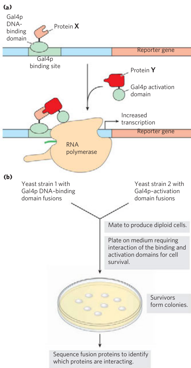
FIGURE 9-21 Yeast two-hybrid analysis. (a) The goal is to bring together the DNA-binding domain and the activation domain of the yeast Gal4 protein (Gal4p) through the interaction of two proteins, X and Y, to which one or other of the domains is fused. This interaction is accompanied by the expression of a reporter gene. (b) The two gene fusions are created in separate yeast strains, which are then mated. The mated mixture is plated on a medium on which the yeast cannot survive unless the reporter gene is expressed. Thus, all surviving colonies have interacting fusion proteins. Sequencing of the fusion proteins in the survivors reveals which proteins are interacting.
