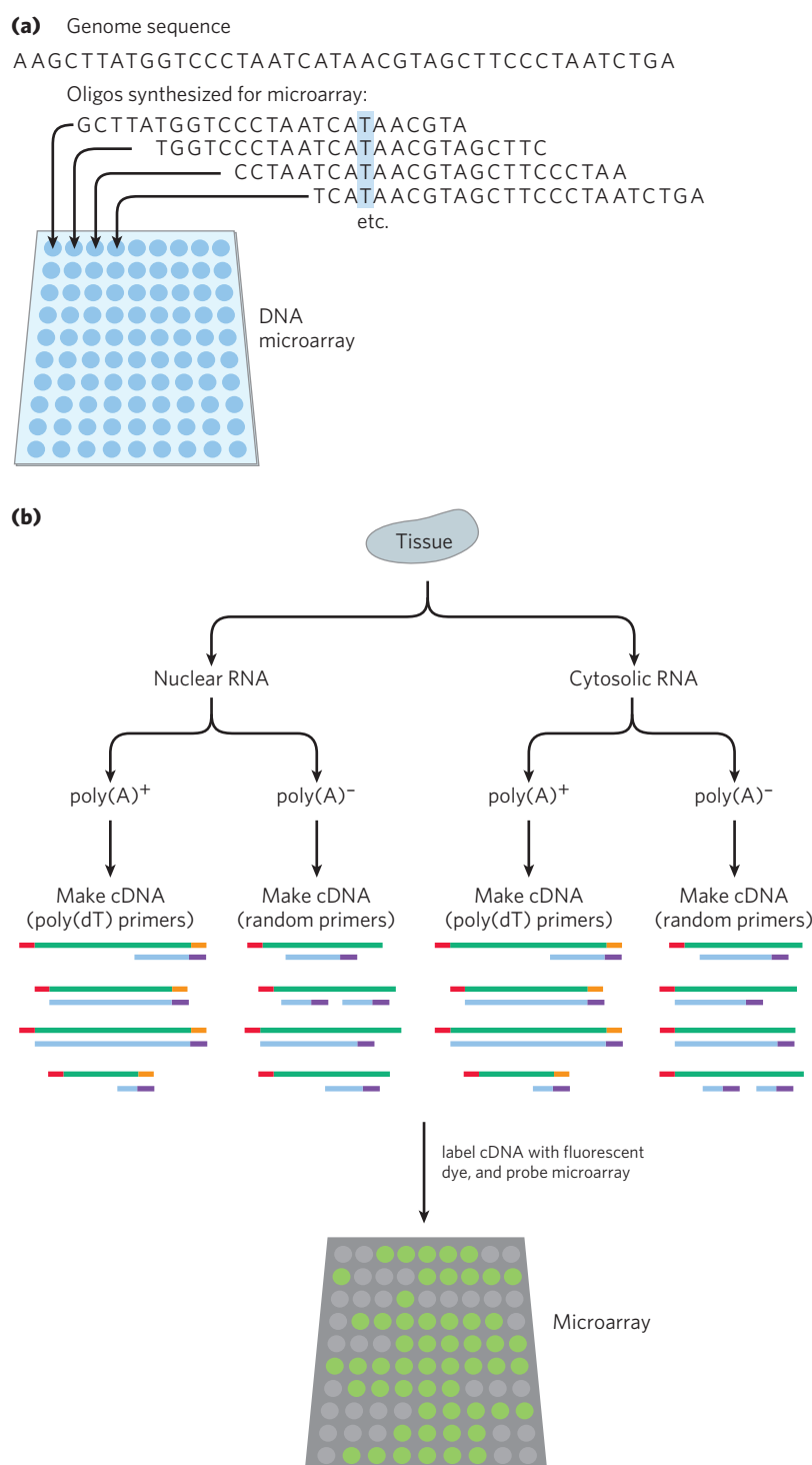
FIGURE 2 Defining the transcriptome with microarrays.
