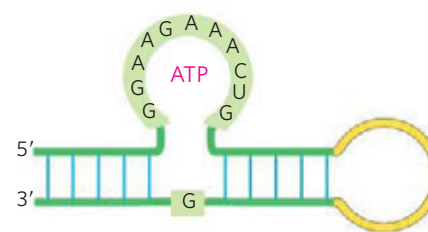
FIGURE 2 RNA aptamer that binds ATP. The shaded nucleotides are those required for the binding activity.
