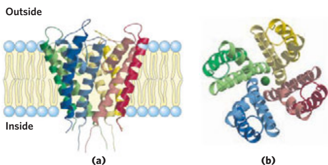
FIGURE 11–47 The K^+ channel of Streptomyces lividans . (PDB ID 1BL8) (a) Viewed in the plane of the membrane, the channel consists of eight transmembrane helices (two from each of four identical subunits), forming a cone with its wide end toward the extracellular space. The inner helices of the cone (lighter colored) line the transmembrane channel, and the outer helices interact with the lipid bilayer. Short segments of each subunit converge in the open end of the cone to make a selectivity filter. (b) This view, perpendicular to the plane of the membrane, shows the four subunits
