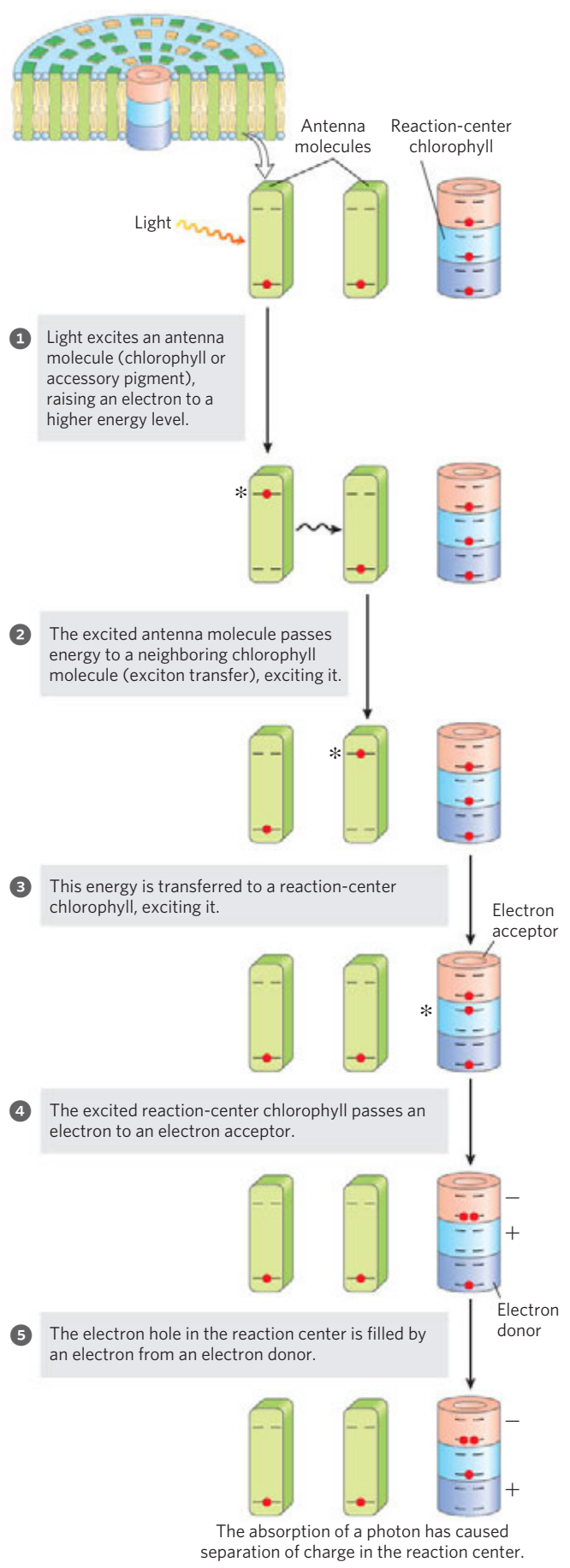
FIGURE 19-54 Organization of photosystems in the thylakoid membrane. Photosystems are tightly packed in the thylakoid membrane, with several hundred antenna chlorophylls and accessory pigments surrounding a photoreaction center. Absorption of a photon by any of the antenna chlorophylls leads to excitation of the reaction center by exciton transfer (red arrow). Also embedded in the thylakoid membrane are the cytochrome b_6f complex and ATP synthase (see Fig. 19-61).
