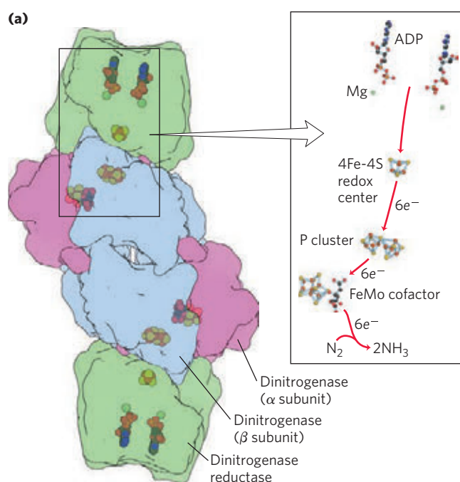
FIGURE 22-3 Enzymes and cofactors of the nitrogenase complex. (PDB ID 1FP6 and PDB ID 1M1N) (a) The holoenzyme consists of two identical dinitrogenase reductase molecules (green), each with a 4Fe-4S redox center and binding sites for two ATP, and two identical dinitrogenase heterodimers (purple and blue), each with a P cluster (Fe-S center) and an FeMo cofactor. In this structure, ADP is bound in the ATP site, to
