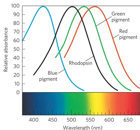
FIGURE 12–40 Absorption spectra of purified rhodopsin and the red, green, and blue receptors of cone cells. The receptor spectra, obtained from individual cone cells isolated from cadavers, peak at about 420, 530, and 560 nm, and the maximum absorption for rhodopsin is at about 500 nm. For reference, the visible spectrum for humans is about 380 to 750 nm.
