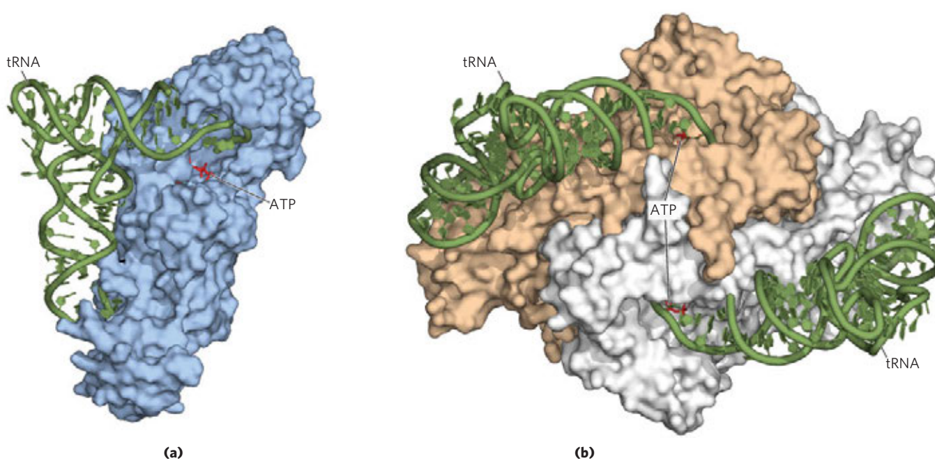
FIGURE 27-22 Aminoacyl-tRNA synthetases. Both synthetases are complexed with their cognate tRNAs (green). Bound ATP (red) pinpoints the active site near the end of the aminoacyl arm. (a) Gln-tRNA synthetase
