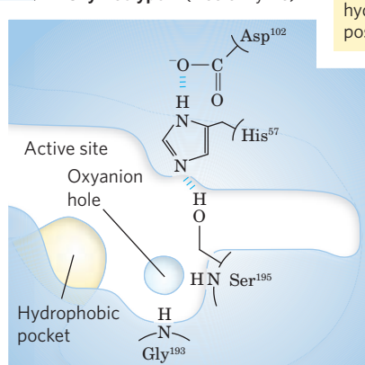
Chymotrypsin (free enzyme)
