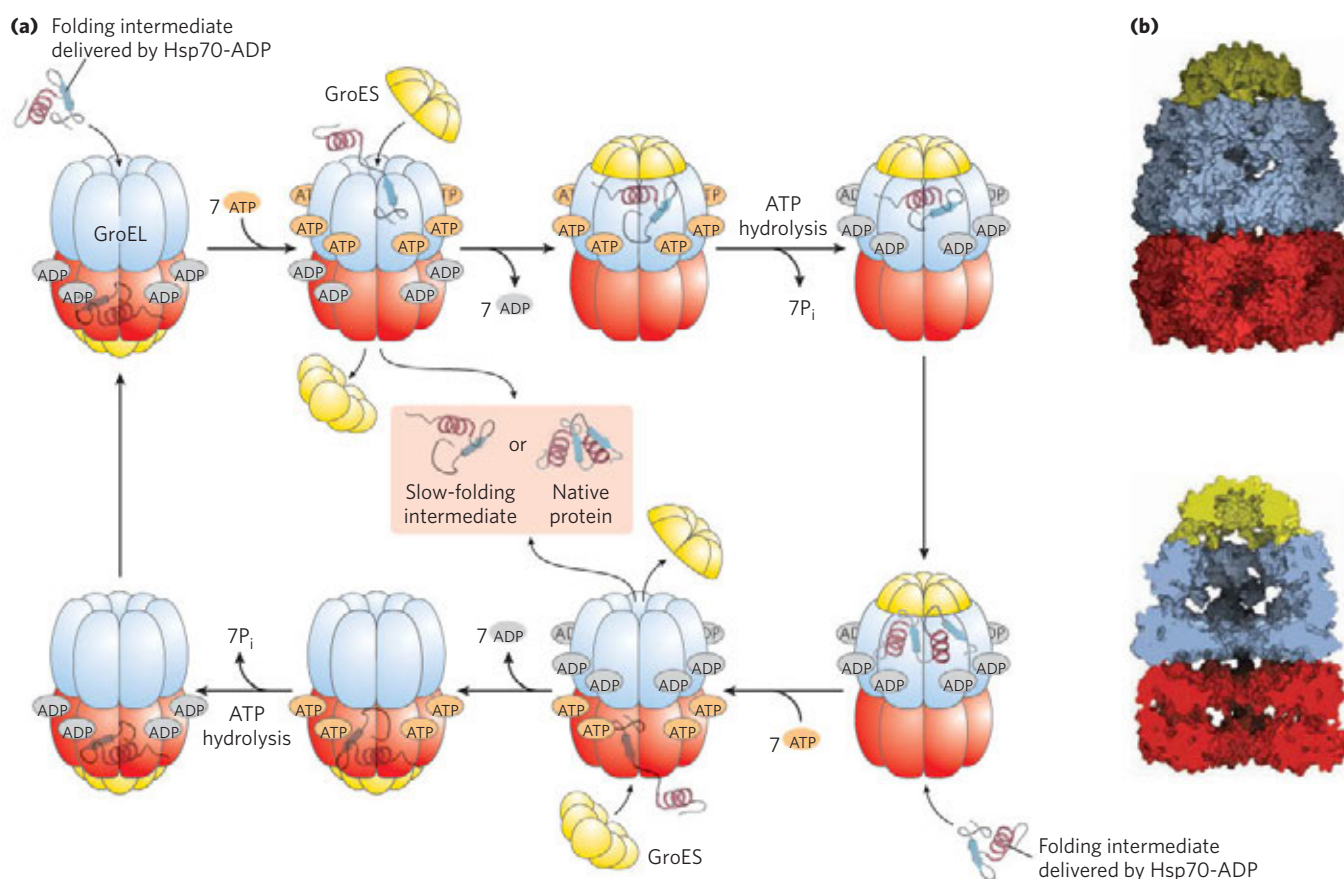
FIGURE 4-31 Chaperonins in protein folding. (a) A proposed pathway for the action of the E. coli chaperonins GroEL (a member of the Hsp60 protein family) and GroES. Each GroEL complex consists of two large chambers formed by two heptameric rings (each subunit M_r 57,000). GroES, also a heptamer (subunit M_r 10,000), blocks one of the GroEL chambers after an unfolded protein is bound inside. The chamber with the unfolded protein is referred to as cis; the opposite one is trans. Folding occurs
