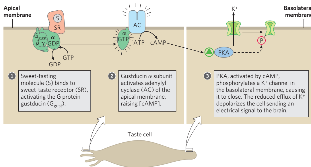
FIGURE 12-42 Transduction mechanism for sweet tastants.
