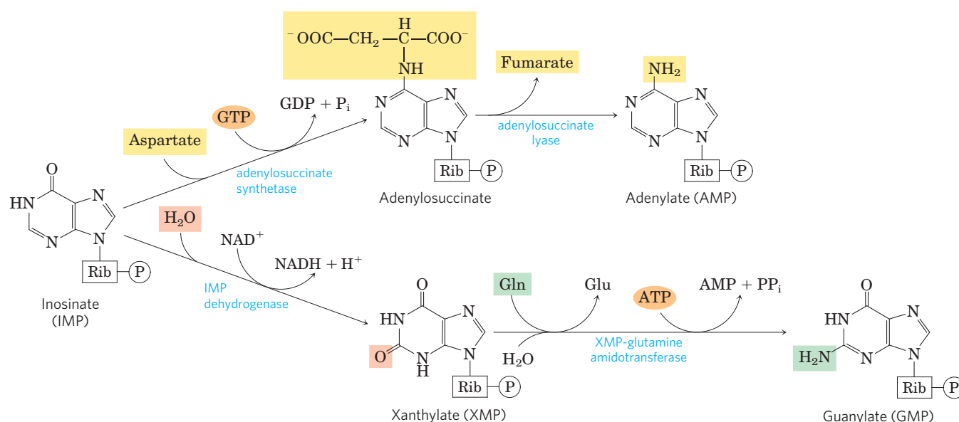
FIGURE 22-36 Biosynthesis of AMP and GMP from IMP.
