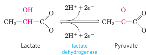
FIGURE 13–10 An oxidation-reduction reaction. Shown here is the oxidation of lactate to pyruvate. In this dehydrogenation, two electrons and two hydrogen ions (the equivalent of two hydrogen atoms) are removed from C-2 of lactate, an alcohol, to form pyruvate, a ketone. In cells the reaction is catalyzed by lactate dehydrogenase and the electrons are transferred to the cofactor nicotinamide adenine dinucleotide (NAD). This reaction is fully reversible; pyruvate can be reduced by electrons transferred from the cofactor.
