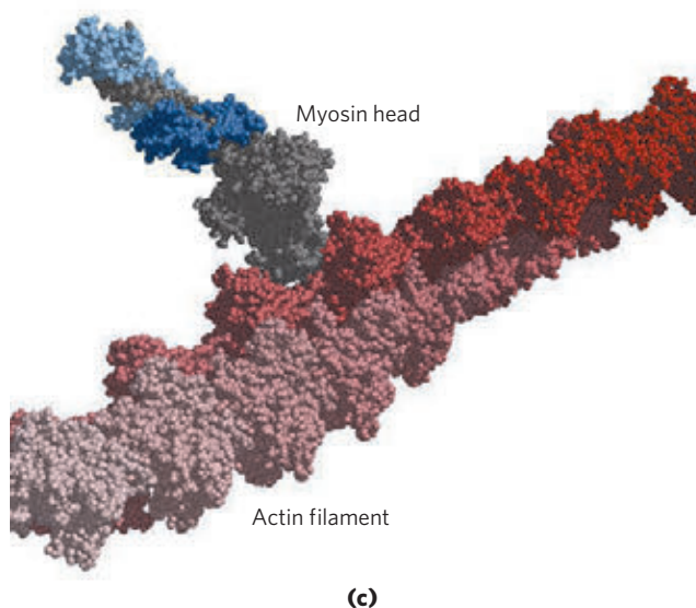
FIGURE 5-28 The major components of muscle. (a) Myosin aggregates to form a bipolar structure called a thick filament. (b) F-actin is a filamentous assemblage of G-actin monomers that polymerize two by two, giving the appearance of two filaments spiraling about one another in a right-handed fashion. (c) Space-filling model of an actin filament (shades of red) with one myosin head (gray and two shades of blue) bound to an actin monomer within the filament (from coordinates supplied by Ivan Rayment).
