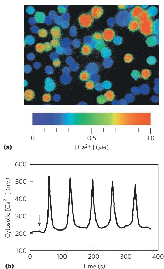
FIGURE 12-12 Triggering of oscillations in intracellular [\text{Ca}^{2+}] by extracellular signals. (a) A dye (fura) that undergoes fluorescence changes when it binds \text{Ca}^{2+} is allowed to diffuse into cells, and its instantaneous light output is measured by fluorescence microscopy. Fluorescence intensity is represented by color; the color scale relates intensity of color to [\text{Ca}^{2+}] , allowing determination of the absolute [\text{Ca}^{2+}] . In this case, thymocytes (cells of the thymus) have been stimulated with extracellular ATP, which raises their internal [\text{Ca}^{2+}] . The cells are heterogeneous in their responses; some have high intracellular [\text{Ca}^{2+}] (red), others much lower (blue). (b) When such a probe is used in a single hepatocyte, the agonist norepinephrine (added at the arrow) causes oscillations of [\text{Ca}^{2+}] from 200 to 500 nM. Similar oscillations are induced in other cell types by other extracellular signals.
