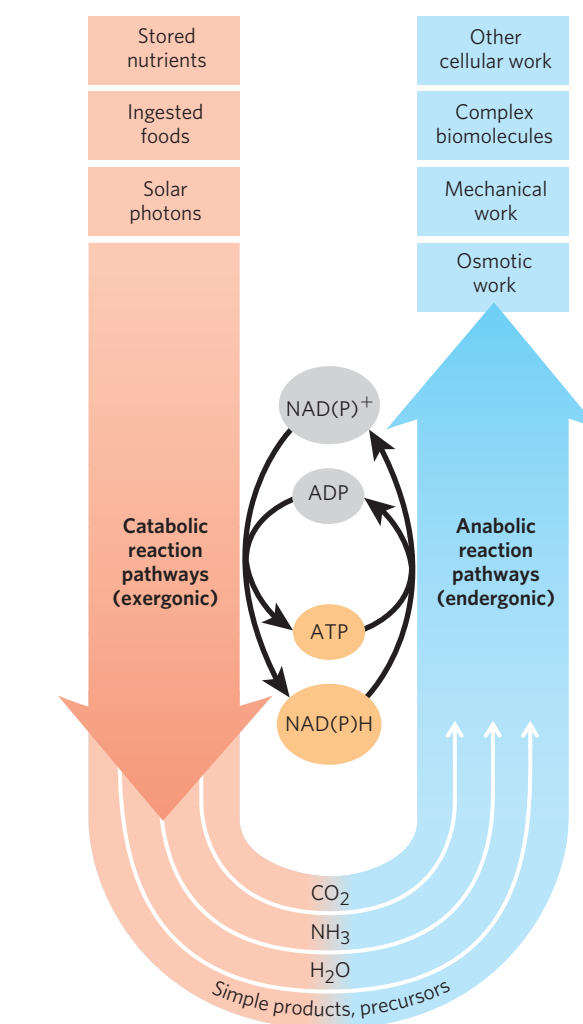
FIGURE 1-29 The central roles of ATP and NAD(P)H in metabolism. ATP is the shared chemical intermediate linking energy-releasing and energy-consuming cellular processes. Its role in the cell is analogous to that of money in an economy: it is “earned/produced” in exergonic reactions and “spent/consumed” in endergonic ones. NAD(P)H (nicotinamide adenine dinucleotide (phosphate)) is an electron-carrying cofactor that collects electrons from oxidative reactions and then donates them in a wide variety of reduction reactions in biosynthesis. Present in relatively low concentrations, these cofactors essential to anabolic reactions must be constantly regenerated by catabolic reactions.
