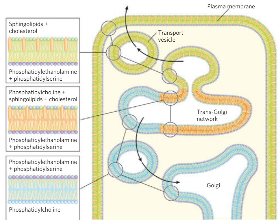
FIGURE 11-6 The distribution of lipids in the membranes of a typical cell. Each membrane has its own characteristic composition, and the
