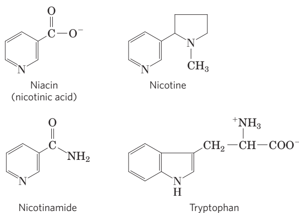
FIGURE 13–26 Niacin (nicotinic acid) and its derivative nicotinamide.
