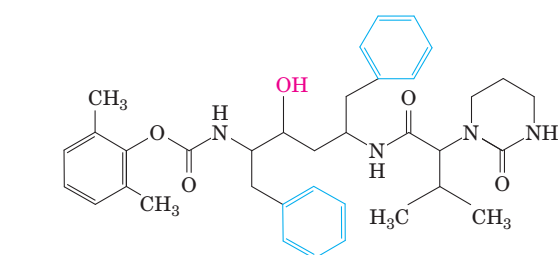
Lopinavir
