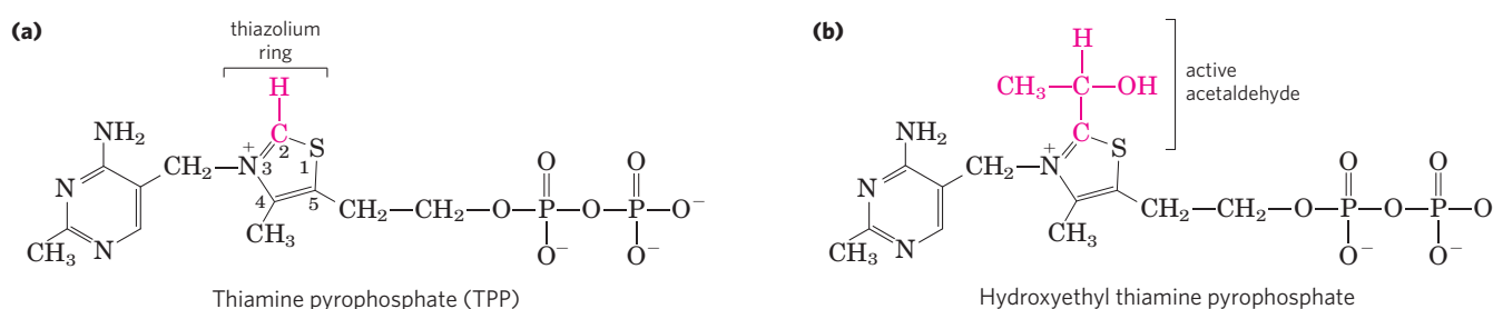
MECHANISM FIGURE 14-15 Thiamine pyrophosphate (TPP) and its role in pyruvate decarboxylation. (a) TPP is the coenzyme form of vitamin B 1 (thiamine). The reactive carbon atom in the thiazolium ring of TPP is shown in red. In the reaction catalyzed by pyruvate decarboxylase, two of the three carbons of pyruvate are carried transiently on TPP in the form of a hydroxyethyl, or “active acetaldehyde,” group (b), which is subsequently released as acetaldehyde. (c) The thiazolium ring of TPP stabilizes carbanion intermediates by providing an electrophilic (electron-deficient) structure into which the carbanion electrons can be delocalized by resonance. Structures with this property, often called “electron sinks,” play a role in many biochemical reactions—here, facilitating carbon-carbon bond cleavage. Thiamine Pyrophosphate Mechanism
