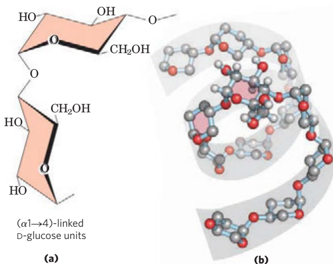
(a) FIGURE 7-19 Helical structure of starch (amylose). (a) In the most stable conformation, with adjacent rigid chairs, the polysaccharide chain is curved, rather than linear as in cellulose (see Fig. 7-14). (b) A model of a segment of amylose; for clarity, the hydroxyl groups have been omitted from all but one of the glucose residues. Compare the two residues shaded in pink with the chemical structures in (a). The conformation of ( \alpha 1 \rightarrow 4 ) linkages in amylose, amylopectin, and glycogen causes these polymers to assume tightly coiled helical structures. These compact structures produce the dense granules of stored starch or glycogen seen in many cells (see Fig. 20-2).
