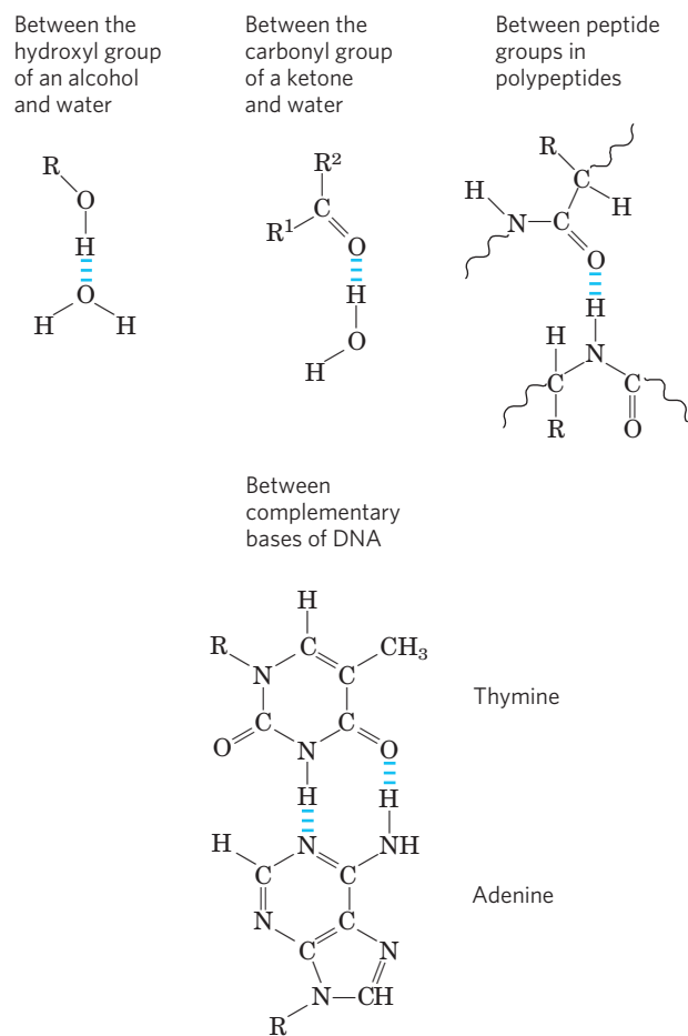
FIGURE 2-4 Some biologically important hydrogen bonds.
