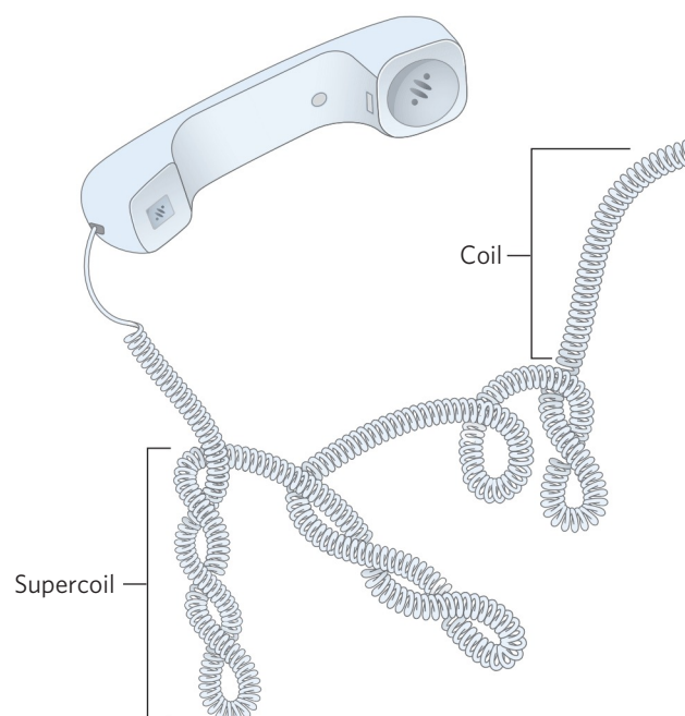
FIGURE 24-9 Supercoils. A typical phone cord is coiled like a DNA helix, and the coiled cord can itself coil in a supercoil. The illustration is especially appropriate because an examination of phone cords helped lead Jerome Vinograd and his colleagues to the insight that many properties of small circular DNAs can be explained by supercoiling. They first detected DNA supercoiling—in small circular viral DNAs—in 1965.
