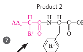
Enzyme-product 2 complex
