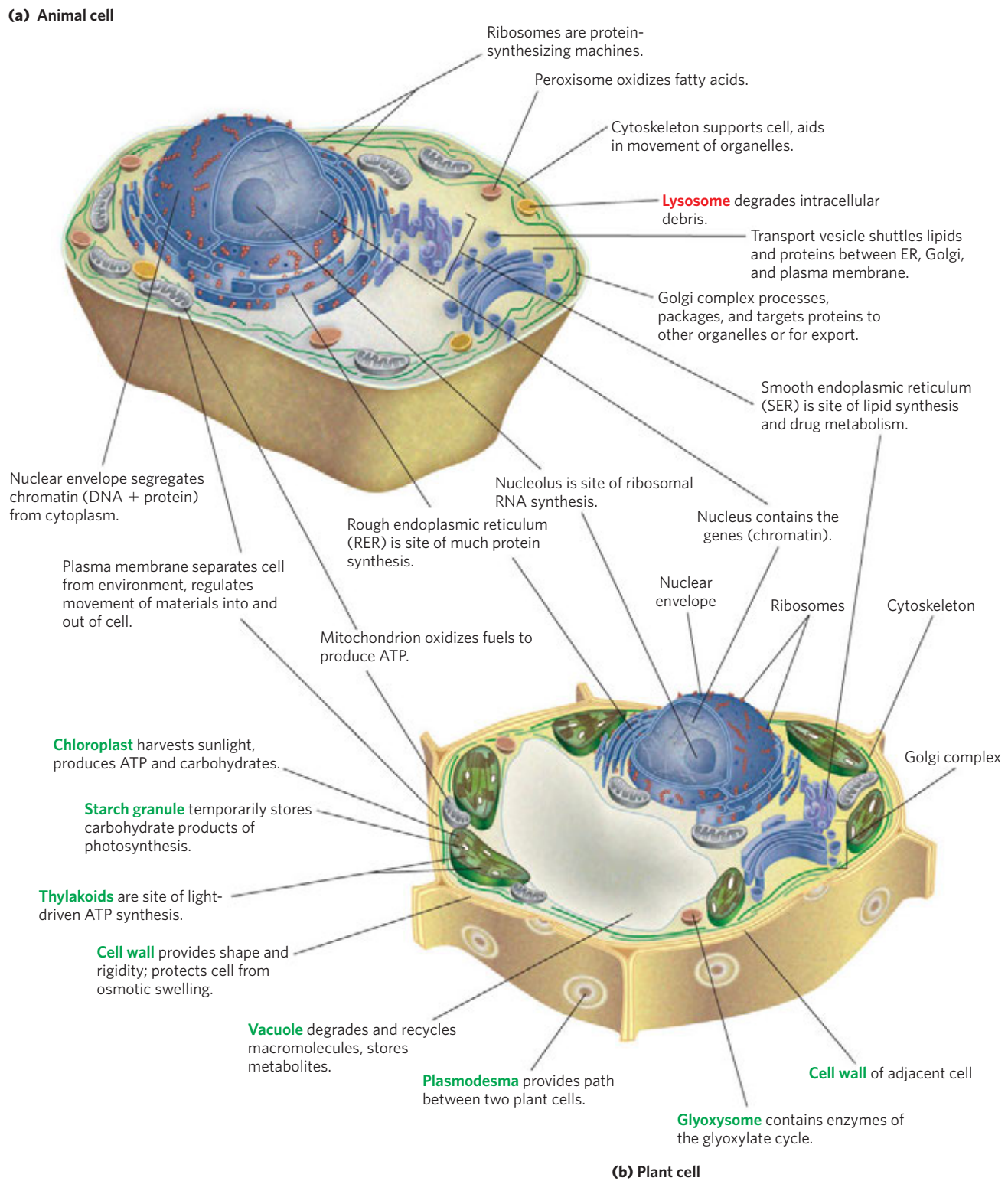
FIGURE 1-7 Eukaryotic cell structure. Schematic illustrations of two major types of eukaryotic cell: (a) a representative animal cell and (b) a representative plant cell. Plant cells are usually 10 to 100 \mu\text{m} in diameter, larger than animal cells, which typically range from 5 to 30 \mu\text{m} . Structures
