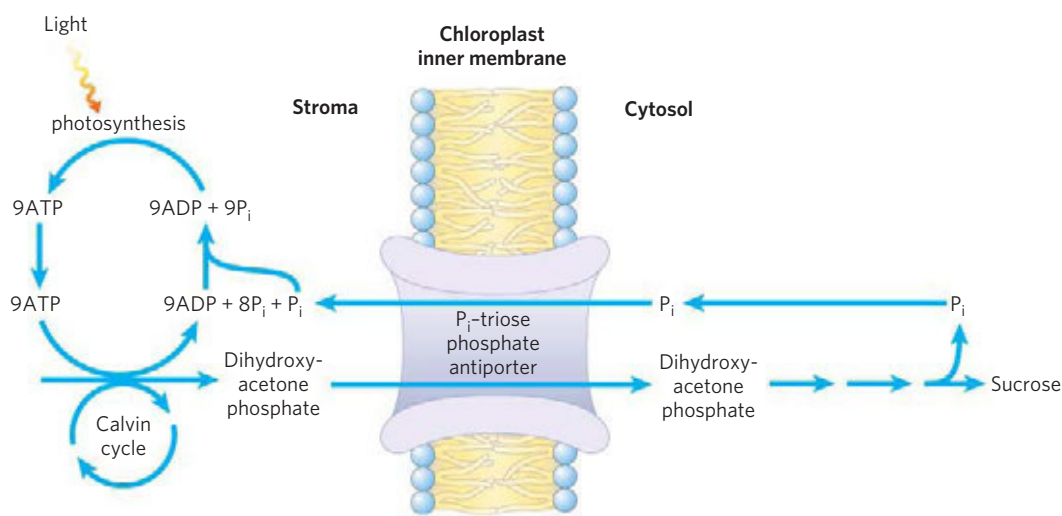
FIGURE 20- chloroplast membrane. This transporter facilitates the exchange of cytosolic \text{P}_i for stromal dihydroxyacetone phosphate. The products of photosynthetic carbon assimilation are thus moved into the cytosol,
