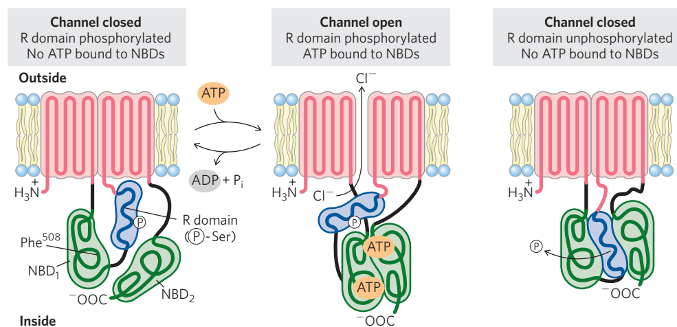
FIGURE 1 Three states of the cystic fibrosis transmembrane conductance regulator, CFTR. The protein has two segments, each with six transmembrane helices, and three functionally significant domains extend from the cytoplasmic surface: NBD 1 and NBD 2 (green) are nucleotide-binding domains that bind ATP, and a regulatory R domain (blue) is the site of phosphorylation by cAMP-dependent protein kinase. When this R domain is phosphorylated but no ATP is bound to the NBDs (left), the channel is closed. The binding of ATP opens the channel (middle) until the bound ATP is hydrolyzed. When the regulatory domain is unphosphorylated (right), it binds the NBD domains and prevents ATP binding and channel opening. The most commonly occurring mutation leading to CF is the deletion of Phe 508 in the NBD 1 domain (left). CFTR is a typical ABC transporter in all but two respects: most ABC transporters lack the regulatory domain, and CFTR acts as an ion channel (for \text{Cl}^- ), not as a typical transporter.
