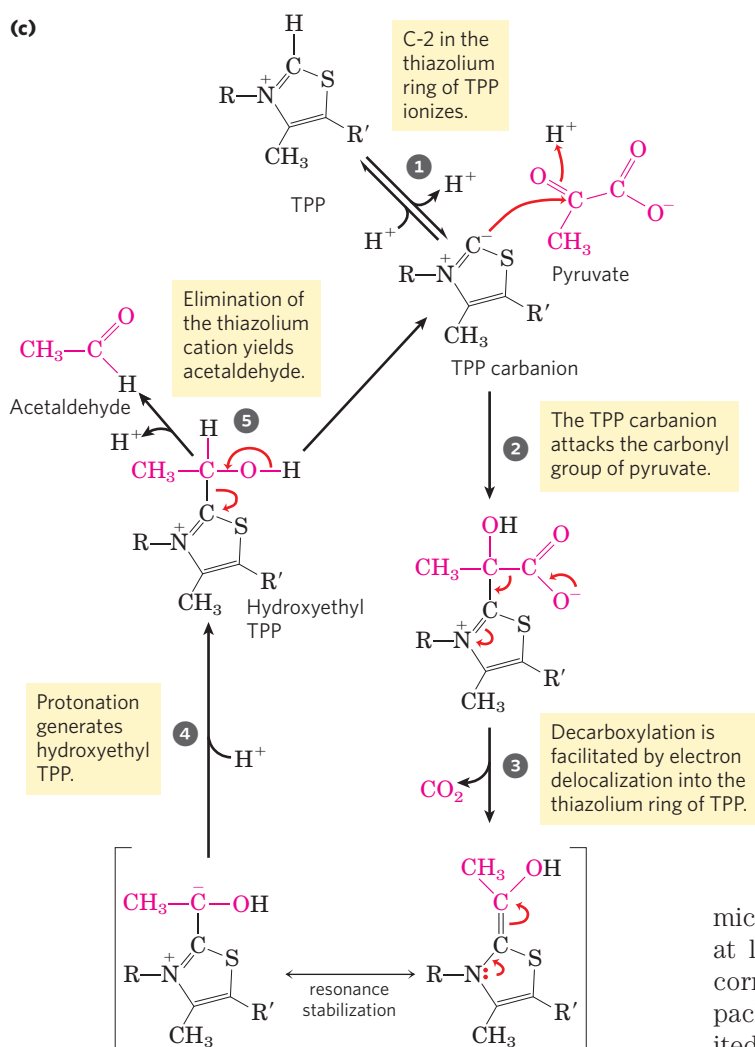
MECHANISM FIGURE 14-15 Thiamine pyrophosphate (TPP) and its role in pyruvate decarboxylation. (a) TPP is the coenzyme form of vitamin B 1 (thiamine). The reactive carbon atom in the thiazolium ring of TPP is shown in red. In the reaction catalyzed by pyruvate decarboxylase, two of the three carbons of pyruvate are carried transiently on TPP in the form of a hydroxyethyl, or “active acetaldehyde,” group (b), which is subsequently released as acetaldehyde. (c) The thiazolium ring of TPP stabilizes carbanion intermediates by providing an electrophilic (electron-deficient) structure into which the carbanion electrons can be delocalized by resonance. Structures with this property, often called “electron sinks,” play a role in many biochemical reactions—here, facilitating carbon-carbon bond cleavage. Thiamine Pyrophosphate Mechanism
