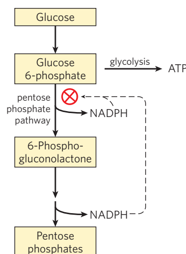
FIGURE 14-28 Role of \text{NADPH} in regulating the partitioning of glucose 6-phosphate between glycolysis and the pentose phosphate pathway. When \text{NADPH} is forming faster than it is being used for biosynthesis and glutathione reduction (see Fig. 14-21), [\text{NADPH}] rises and inhibits the first enzyme in the pentose phosphate pathway. As a result, more glucose 6-phosphate is available for glycolysis.
