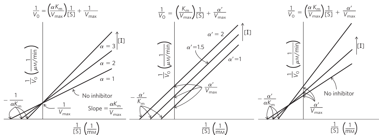
FIGURE 1 Competitive inhibition.
