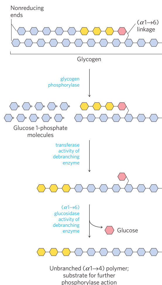
FIGURE 15–28 Glycogen breakdown near an (α1→6) branch point.
