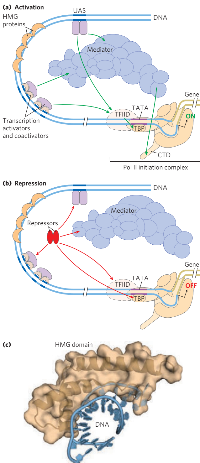
FIGURE 28–28 Eukaryotic promoters and regulatory proteins. RNA polymerase II and its associated basal (general) transcription factors form a pre-initiation complex at the TATA box and Inr site of the cognate promoters, a process facilitated by transcription activators, acting through coactivators (Mediator, TFIID, or both). (a) A composite promoter with typical sequence elements and protein complexes found in both yeast and higher eukaryotes. The carboxyl-terminal domain (CTD) of Pol II (see Fig. 26–9) is an important point of interaction with Mediator and other protein complexes. Histone modification enzymes (not shown) catalyze methylation and acetylation; remodeling enzymes alter the content and placement of nucleosomes. The transcription activators have distinct DNA-binding domains and activation domains. Green arrows indicate common modes of interaction often required for the activation of transcription, as discussed in the text. The HMG proteins are a common type of architectural regulator (see Fig. 28–5), facilitating the looping of the DNA required to bring together system components bound at distant binding sites. (b) Eukaryotic transcriptional repressors function by a range of mechanisms. Some bind directly to DNA, displacing a protein complex required for activation (not shown); many others interact with various parts of the transcription or activation protein complexes to prevent activation. Possible points of interaction are indicated with red arrows. (c) The structure of an HMG protein complex with DNA shows how HMG proteins facilitate DNA looping. The binding is relatively nonspecific, although DNA sequence preferences have been identified for many HMG proteins. Shown is the HMG domain of the protein HMG-D of Drosophila , bound to DNA (PDB ID 1QRV).
