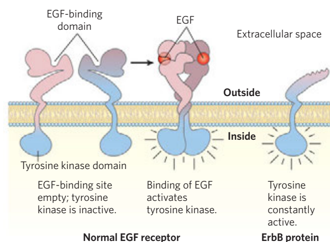
FIGURE 12–50 Oncogene-encoded defective EGF receptor. The product of the erbB oncogene (the ErbB protein) is a truncated version of the normal receptor for epidermal growth factor (EGF). Its intracellular domain has the structure normally induced by EGF binding, but the protein lacks the extracellular binding site for EGF. Unregulated by EGF, ErbB continuously signals cell division.
