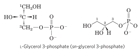
FIGURE 10-8 L-Glycerol 3-phosphate, the backbone of phospholipids.
