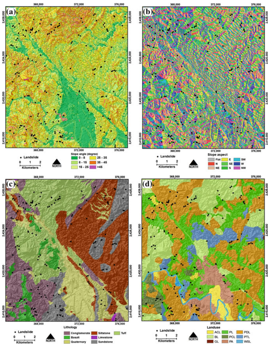
Fig. 2 a Slope; b Aspect; c Lithology; d Land use (ACL annual crop land; BL barren land; GL grass land; P paddy land; PCL perennial crop land; PA populated area; PDL productive forest land; PTL protective forest land; WSL water surface land)
