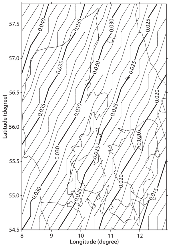
Fig. 5.9. Earth tide displacement (in meters) in Denmark (Dec. 31, 1998; GPS time 1:00; height component)
