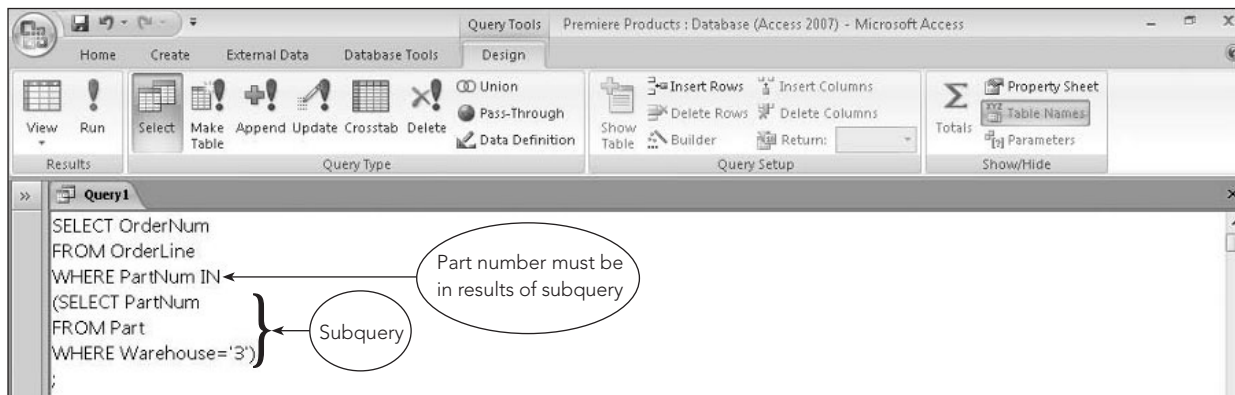
FIGURE 3-40 SQL query with a subquery
