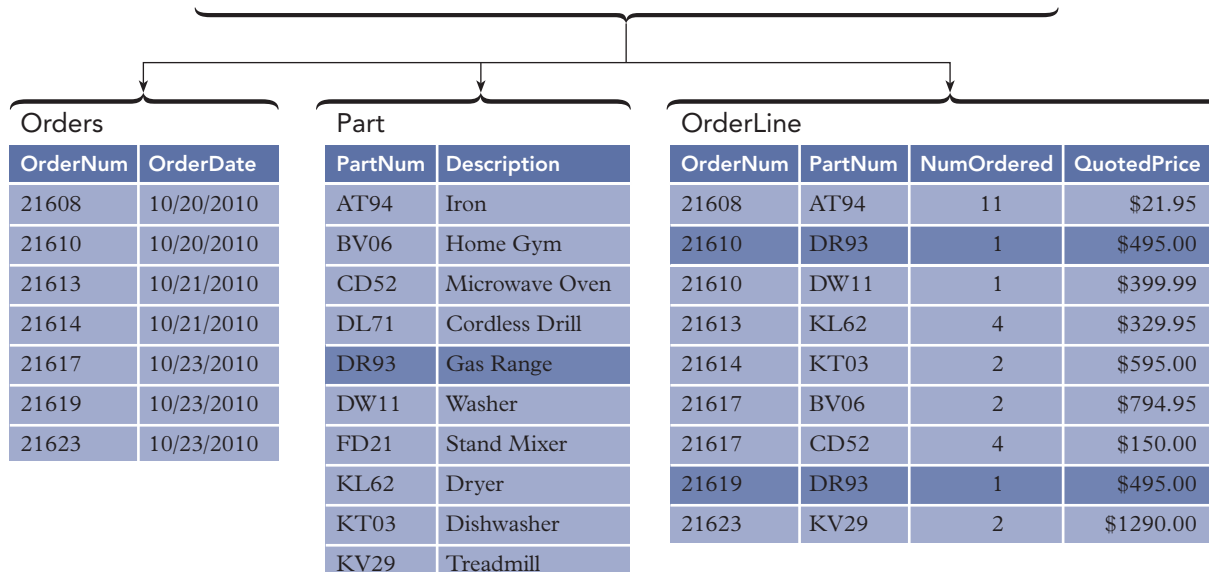
FIGURE 5-9 Conversion to second normal form
