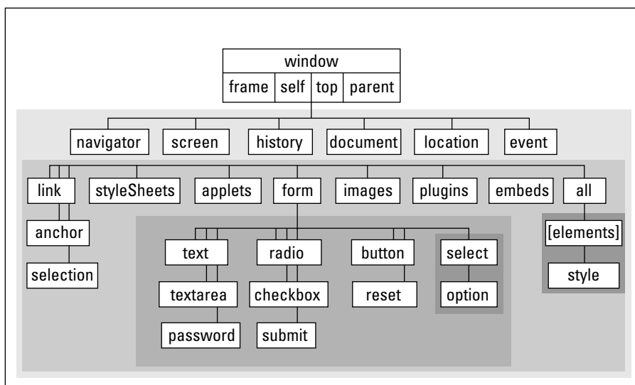
Figure 14-2: The IE4 document object hierarchy
