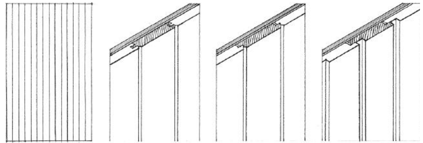
Matched Siding
