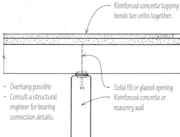
Bearing Wall
