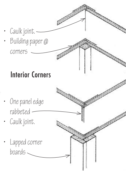
Exterior Corners
