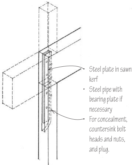
Concealed Connection
