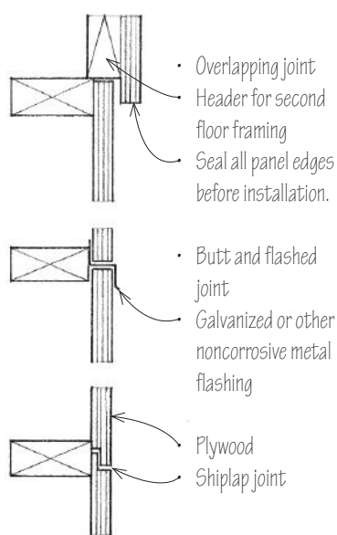
Horizontal Joints
