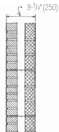
10" (255) Cavity Wall
