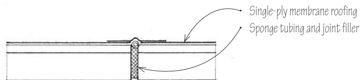
Flat Roof
