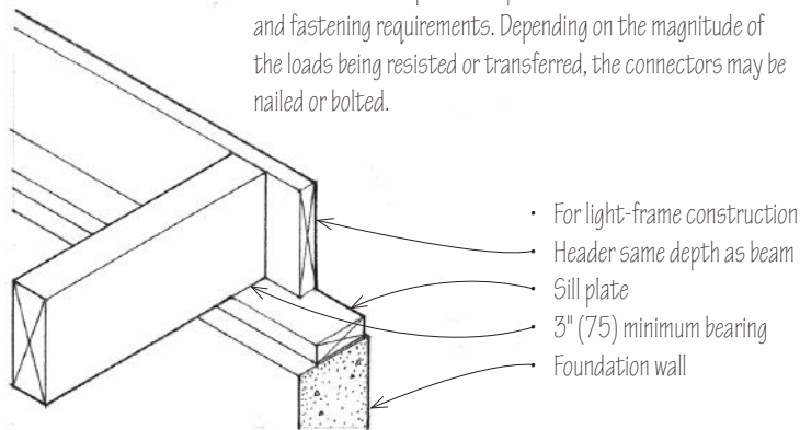
Foundation Wall Support
