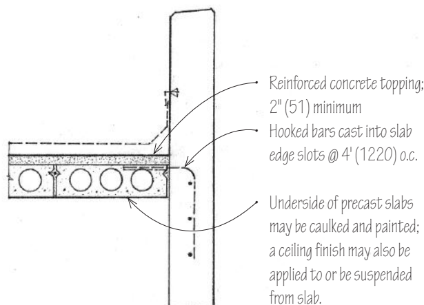
End Wall
