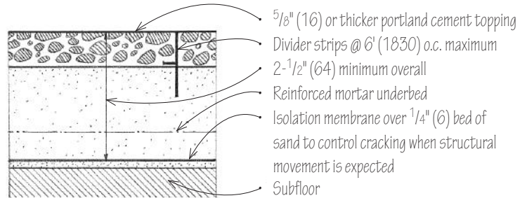
Sand-Cushion Terrazzo
