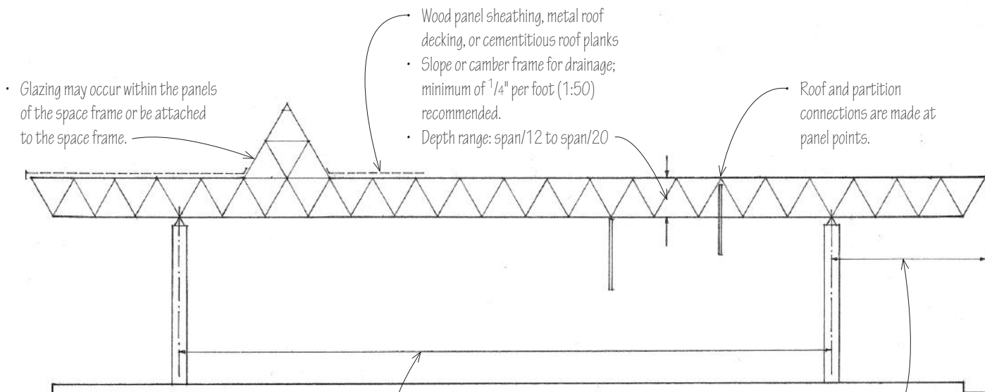
• Interior wall • Exterior wall
