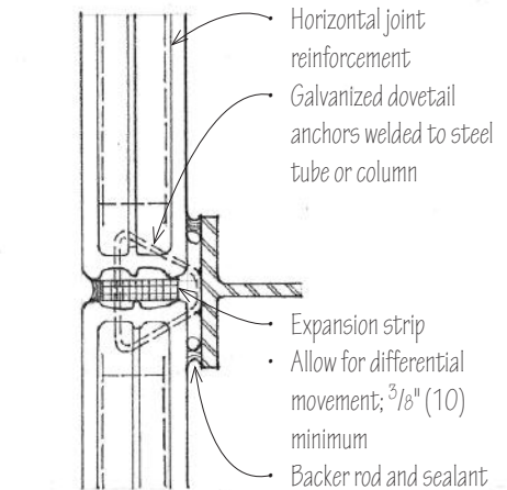
Vertical Stiffener
