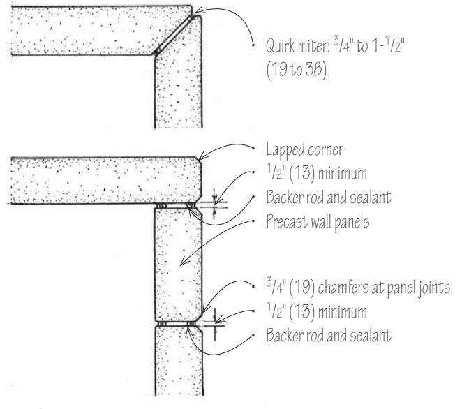
Panel Connections
