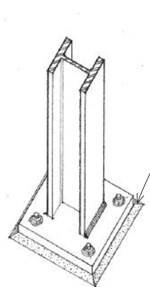
• Column is welded to its steel base plate after the plate is leveled on a bed of nonshrinking grout.
