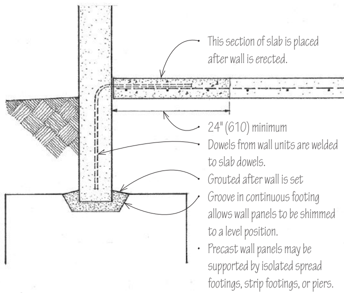
Foundations
