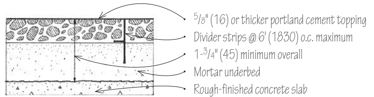
Bonded Terrazzo
