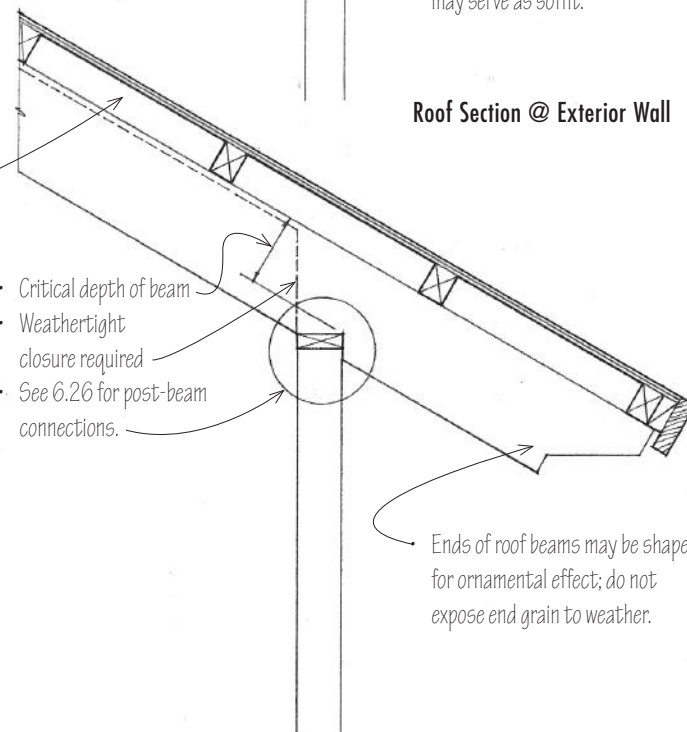
Roof Section @ Exterior Wall
