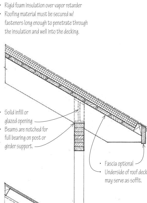
Roof Section @ Exterior Wall
