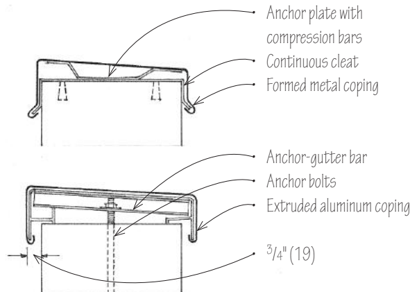
Metal Copings
