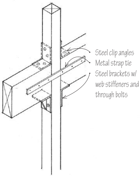
Continuous Post
