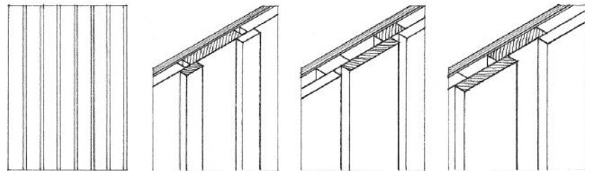
Board Siding
