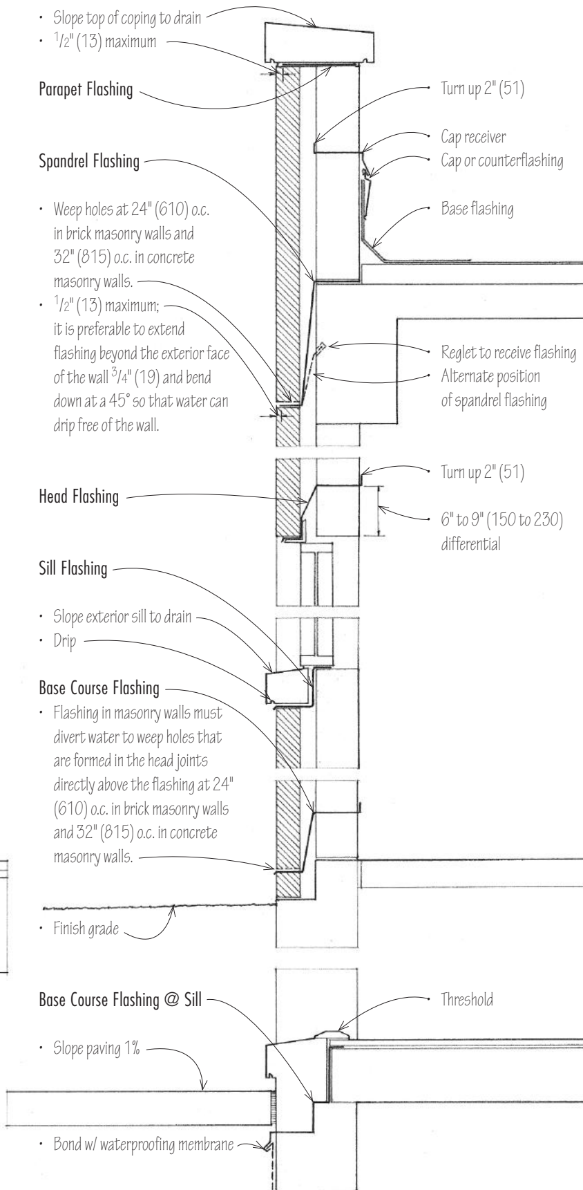
Masonry Wall
