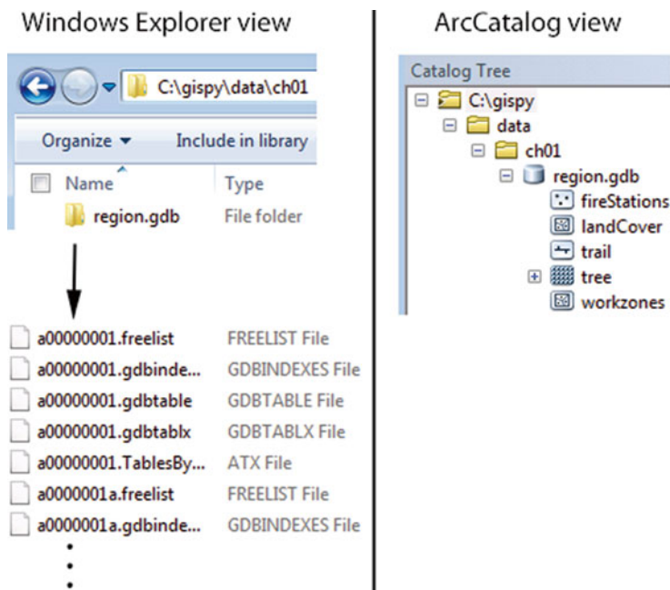
Figure 1.3 Windows Explorer and ArcCatalog views of an Esri file geodatabase, 'region.gdb'.
