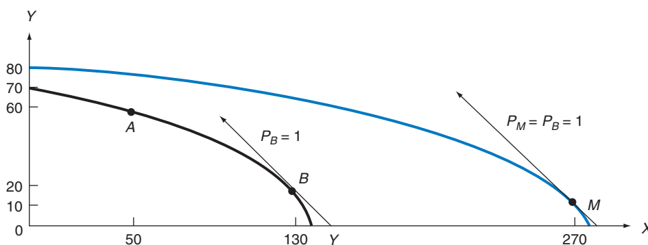
FIGURE 7.2. The Growth of Labor Only and the Rybczynski Theorem. With trade but before growth, Nation 1 produces at point B (130X and 20Y) at P_X/P_Y = P_B = 1 , as in previous chapters. After only L doubles and with P_X/P_Y remaining at P_B = 1 , Nation 1 produces at point M (270X and 10Y) on its new and expanded production frontier. Thus, the output of X (the L -intensive commodity) expanded, and the output of Y (the K -intensive commodity) declined, as postulated by the Rybczynski theorem.
