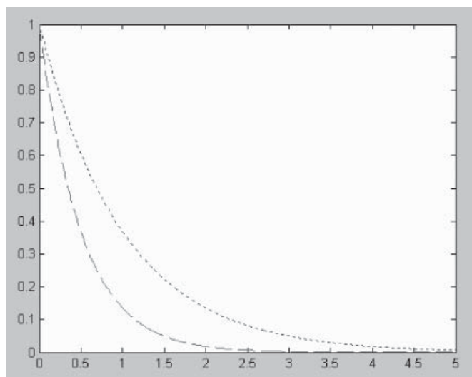
Figure 3-10 Using a dotted line to represent f(t) = e^{-t} and a dashed line to represent g(t) = e^{-2t}
