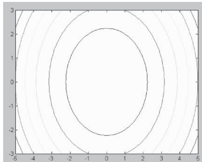
Figure 3-37 A contour plot of z = x^2 + y^2
