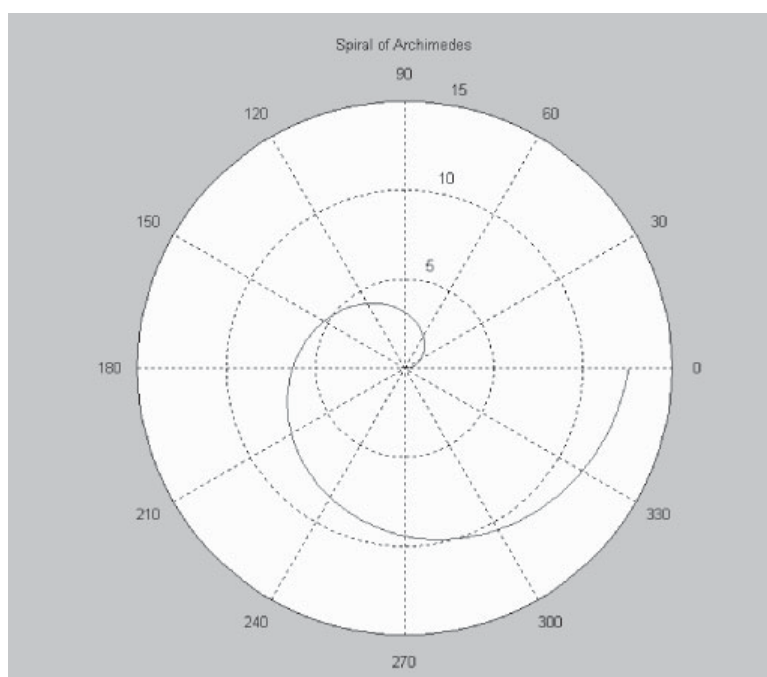
Figure 3-26 A polar plot of the spiral of Archimedes
