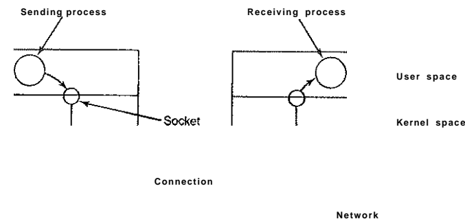
Figure 10-19. The uses of sockets for networking.
