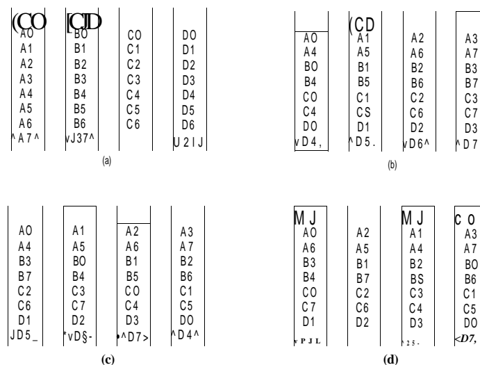
Figure 7-24. Four ways of organizing multimedia files over multiple disks, (a) No striping, (b) Same striping pattern for all files, (c) Staggered striping, (d) Random striping.
