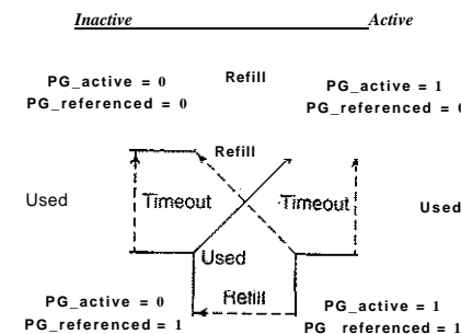
Figure 10-18. Page states considered in the page frame replacement algorithm.
