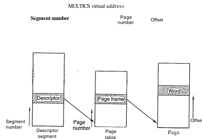
Figure 3-37. Conversion of a two-part MULTICS address into a main memory address.
