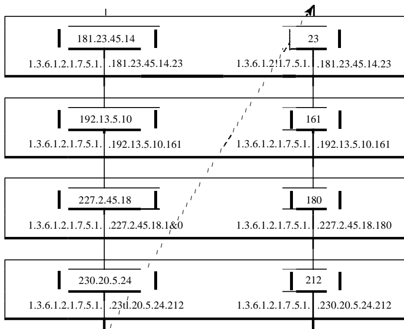
Figure 28.19 Lexicographic ordering
