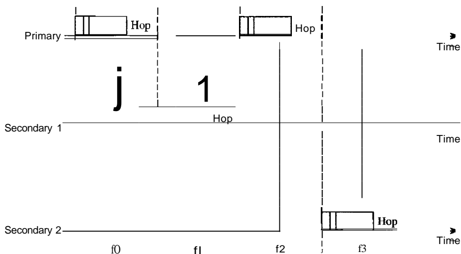
Figure 14.23 Multiple-secondary communication
