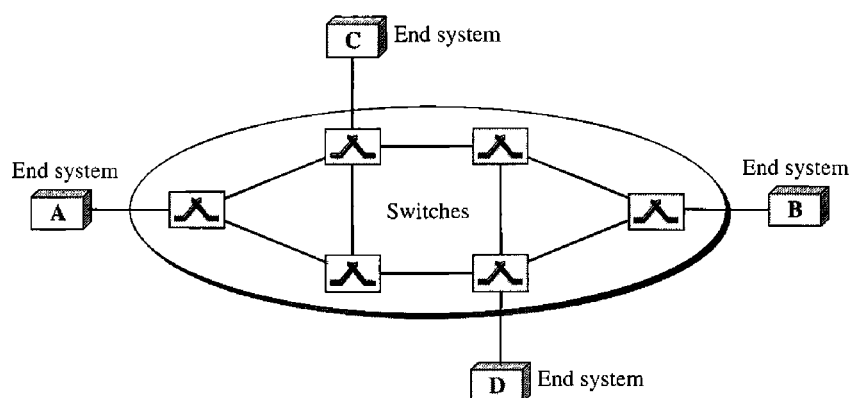
Figure 8.10 Virtual-circuit network
