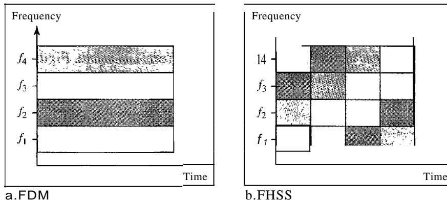
Figure 6.31 Bandwidth sharing
