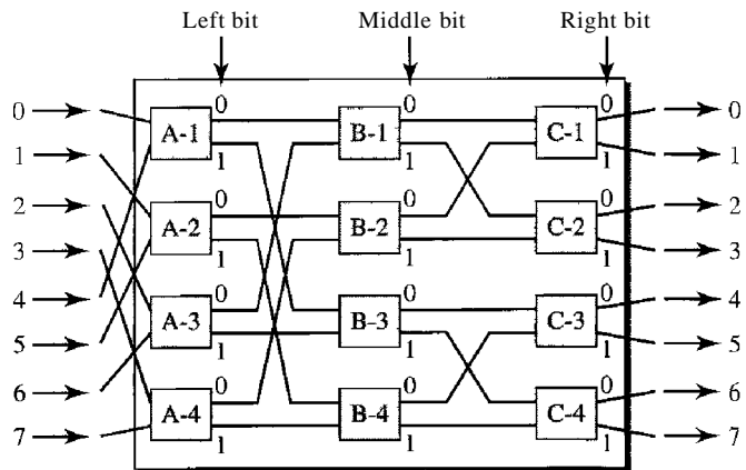
Figure 8.24 A banyan switch
