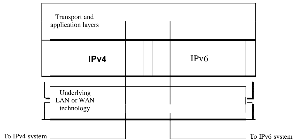
Figure 20.19 Dual stack
