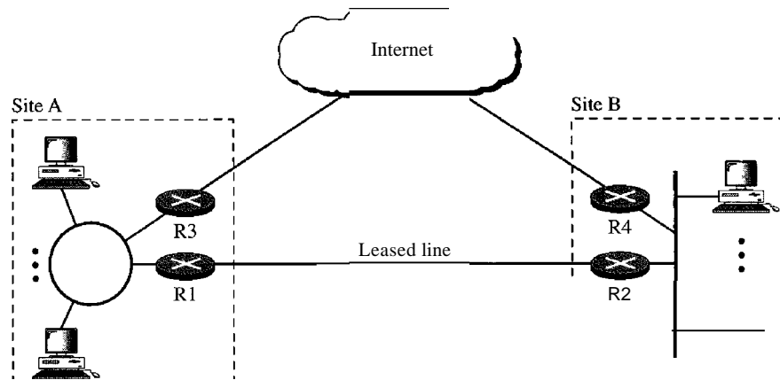
Figure 32.11 Hybrid network
