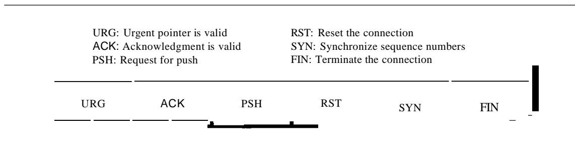
Figure 23.17 Control field
