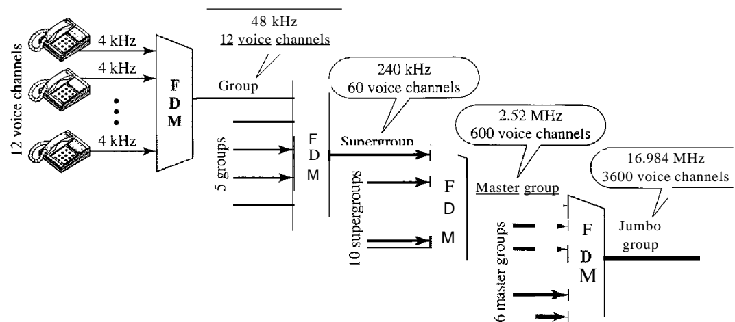
Figure 6.9 Analog hierarchy
