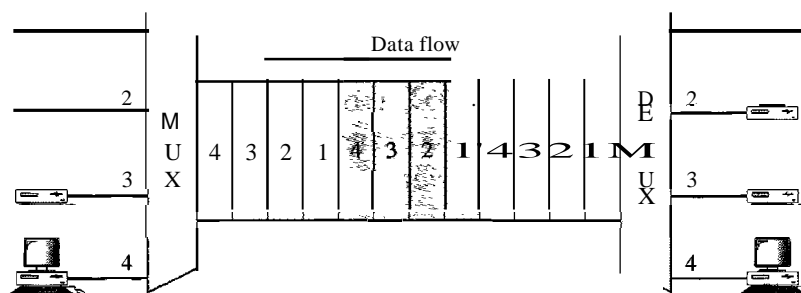
Figure 6.12 TDM
