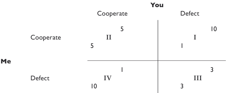
Figure 7.2 Pay-off matrix for a “tit for tat” experiment. Entries in cells show benefit received. (See text for details.)
