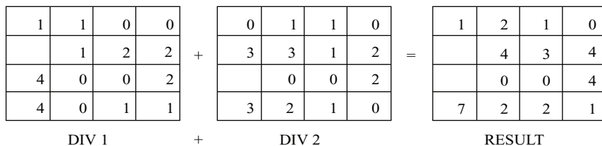
FIGURE 6.12 Arithmetic operators
