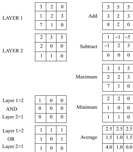
FIGURE 6.11 Raster overlay
