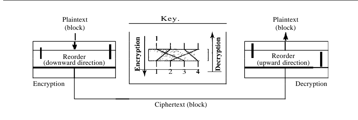
Figure 30.8 Transposition cipher
