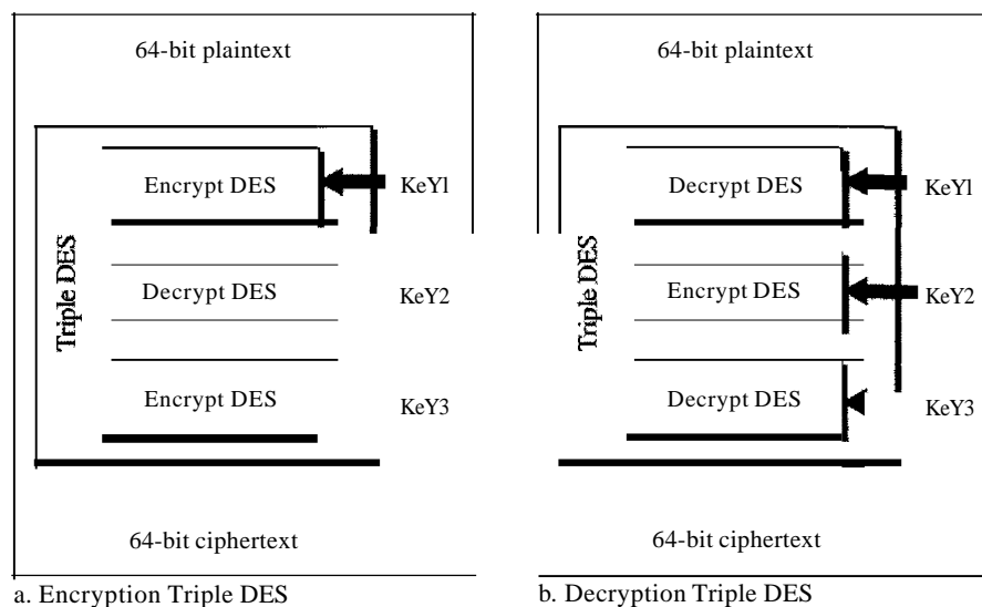
Figure 30.16 Triple DES
