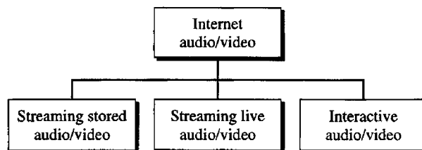
Figure 29.1 Internet audio/video
