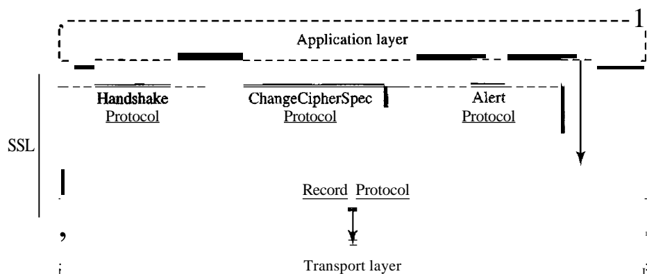
Figure 32.16 Four SSL protocols
