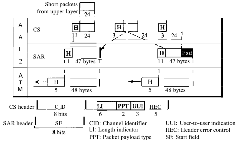
Figure 18.21 AAL2
