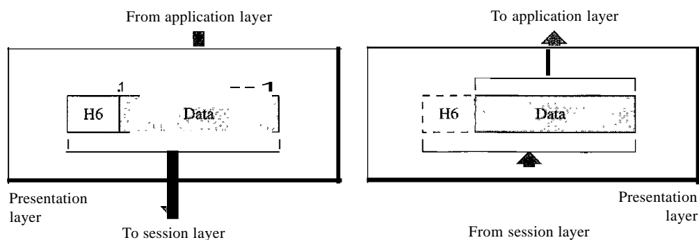
Figure 2.13 Presentation layer
