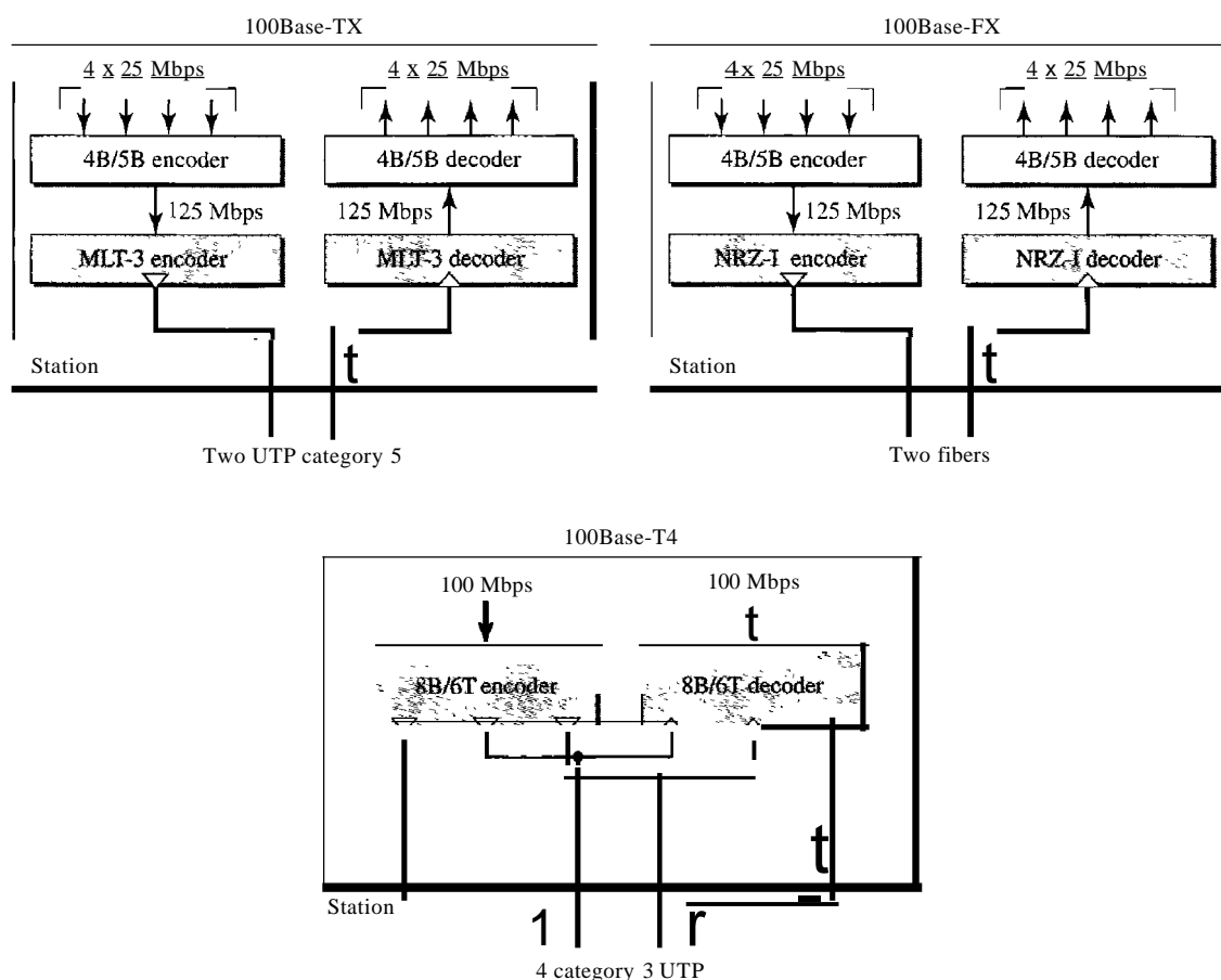
Figure 13.21 Encoding for Fast Ethernet implementation
