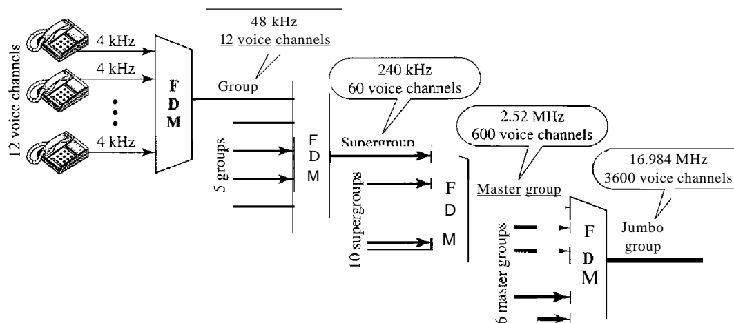
Figure 6.9 Analog hierarchy
