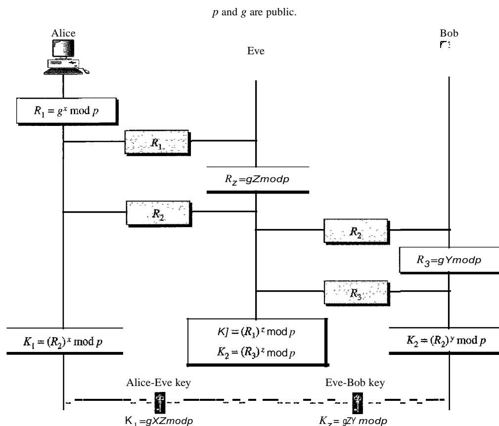
Figure 30.28 Man-in-the-middle attack
