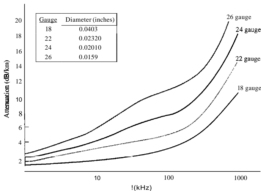
Figure 7.6 UTP performance
