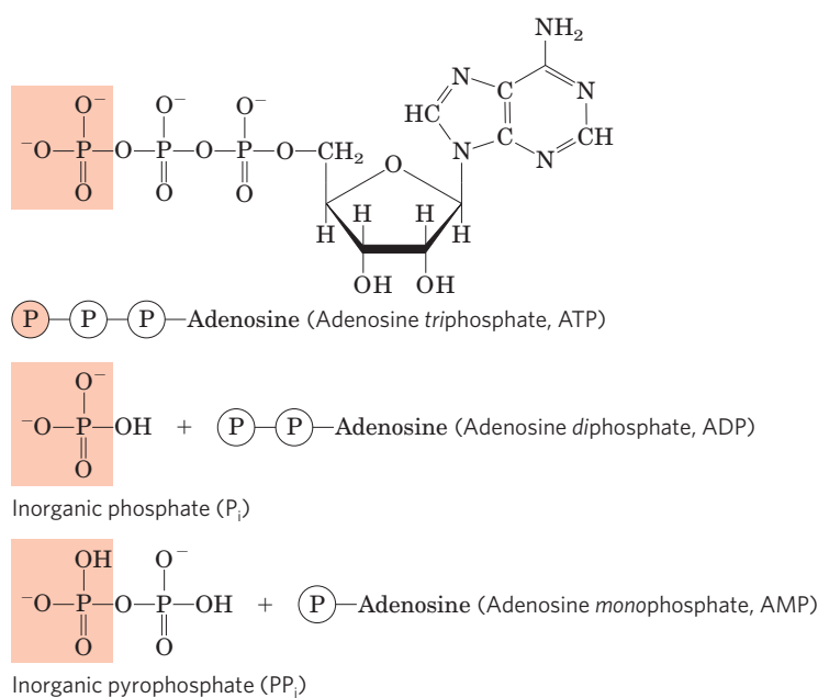
FIGURE 1-26 Adenosine triphosphate (ATP) provides energy. Here, each \textcircled{\text{P}} represents a phosphoryl group. The removal of the terminal phosphoryl group (shaded light red) of ATP, by breakage of a phosphoanhydride bond to generate adenosine diphosphate (ADP) and inorganic phosphate ion ( \text{HPO}_4^{2-} ), is highly exergonic, and this reaction is coupled to many endergonic reactions in the cell (as in the example in Fig. 1-27b). ATP also provides energy for many cellular processes by undergoing cleavage that releases the two terminal phosphates as inorganic pyrophosphate ( \text{H}_2\text{P}_2\text{O}_7^{2-} ), often abbreviated \text{PP}_i .
