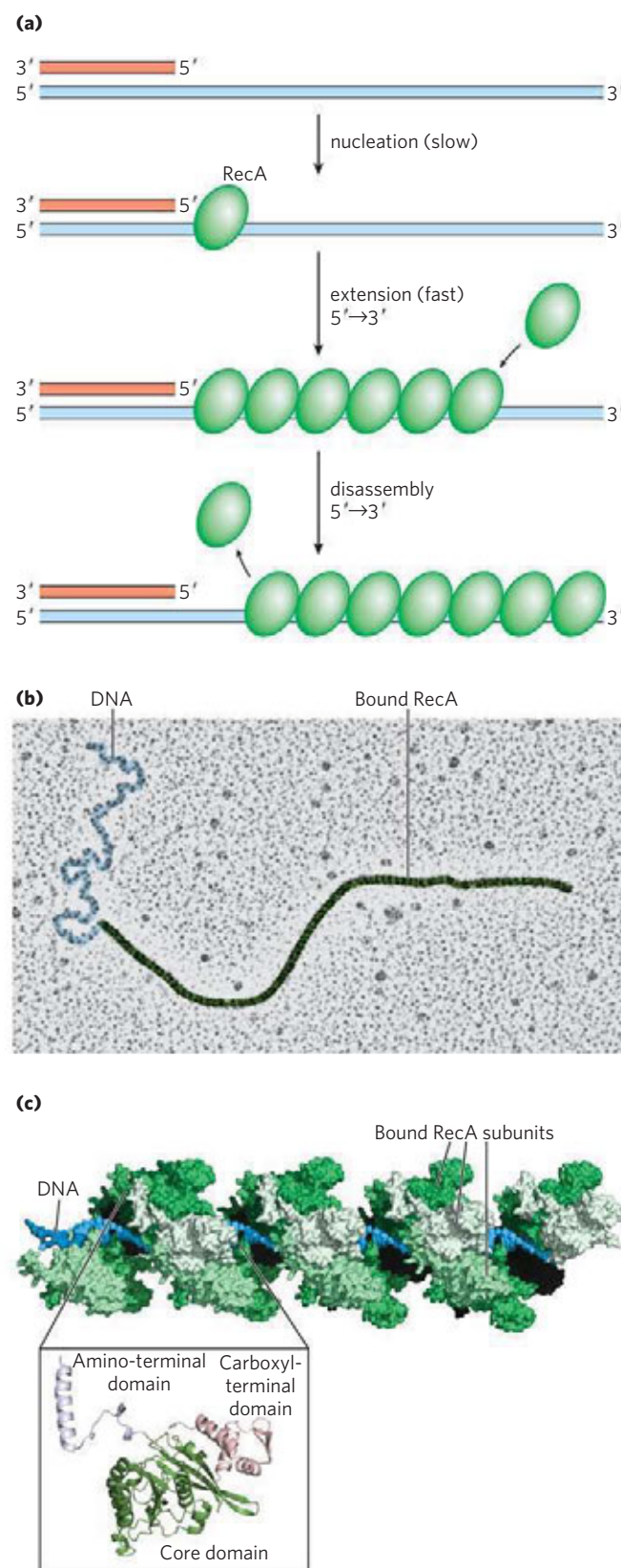
FIGURE 25–32 RecA protein filaments. RecA and other recombinases in this class function as filaments of nucleoprotein. (a) Filament formation proceeds in discrete nucleation and extension steps. Nucleation is the addition of the first few RecA subunits. Extension occurs by adding RecA subunits so that the filament grows in the 5′→3′ direction. When disassembly occurs, subunits are subtracted from the trailing end. (b) Colorized electron micrograph of a RecA filament bound to DNA. (c) Segment of a RecA filament with four helical turns (24 RecA subunits; derived from PDB ID 3CMX). Notice the bound double-stranded DNA in the center. The core domain of RecA is structurally related to the domains in helicases.
