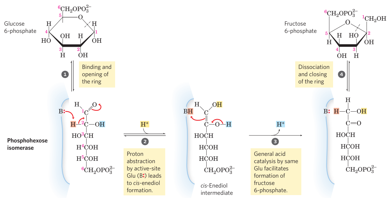
MECHANISM FIGURE 14-5 The phosphohexose isomerase reaction. The ring opening and closing reactions (steps 1 and 4) are catalyzed by an active-site His residue, by mechanisms omitted here for simplicity. The proton (light red) initially at C-2 is made more easily abstractable by electron withdrawal by the adjacent carbonyl and nearby hydroxyl
