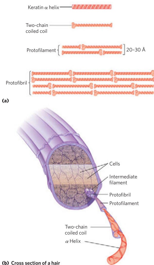
FIGURE 4-11 Structure of hair. (a) Hair α-keratin is an elongated α helix with somewhat thicker elements near the amino and carboxyl termini. Pairs of these helices are interwound in a left-handed sense to form two-chain coiled coils. These then combine in higher-order structures called protofilaments and protofibrils. About four protofibrils—32 strands of α-keratin in all—combine to form an intermediate filament. The individual two-chain coiled coils in the various substructures also seem to be interwound, but the handedness of the interwinding and other structural details are unknown. (b) A hair is an array of many α-keratin filaments, made up of the substructures shown in (a).
