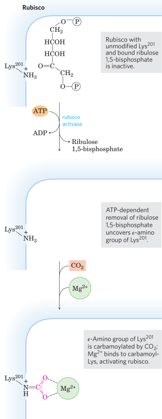
FIGURE 20-8 Role of rubisco activase in the carbamoylation of Lys 201 of rubisco. When the substrate ribulose 1,5-bisphosphate is bound to the active site, Lys 201 is not accessible. Rubisco activase couples ATP hydrolysis to expulsion of the bound sugar bisphosphate, exposing Lys 201 ; this Lys residue can now be carbamoylated with CO 2 in a reaction that is apparently not enzyme-mediated. Mg 2+ is attracted to and binds to the negatively charged carbamoyl-Lys, and the enzyme is thus activated.
