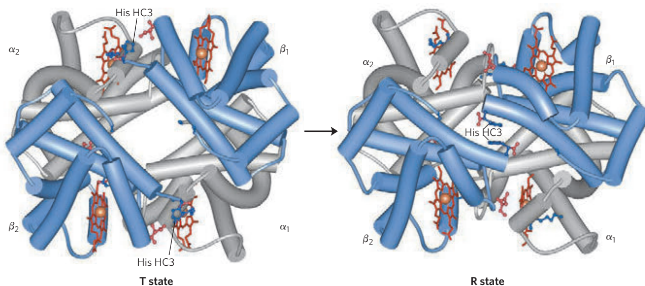
FIGURE 5-10 The T → R transition. (PDB ID 1HGA and 1BBB) In these depictions of deoxyhemoglobin, as in Figure 5-9, the β subunits are blue and the α subunits are gray. Positively charged side chains and chain termini involved in ion pairs are shown in blue, their negatively charged partners in red. The Lys C5 of each α subunit and Asp FG1 of each β subunit are visible but not labeled (compare Fig. 5-9a). Note that the molecule is oriented slightly differently than in Figure 5-9. The
