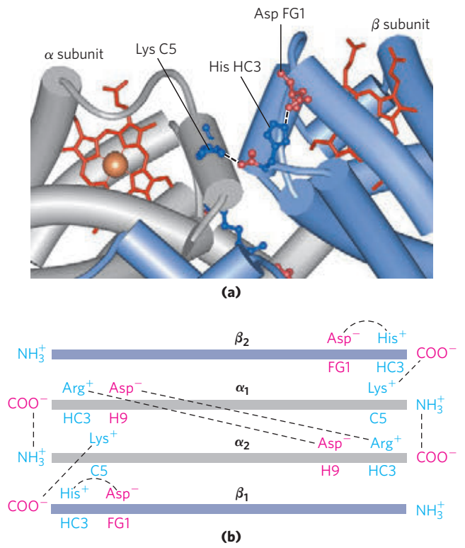
FIGURE 5-9 Some ion pairs that stabilize the T state of deoxyhemoglobin. (a) Close-up view of a portion of a deoxyhemoglobin molecule in the T state (PDB ID 1HGA). Interactions between the ion pairs His HC3 and Asp FG1 of the \beta subunit (blue) and between Lys C5 of the \alpha subunit (gray) and His HC3 (its \alpha -carboxyl group) of the \beta subunit are shown with dashed lines. (Recall that HC3 is the carboxyl-terminal residue of the \beta subunit.) (b) Interactions between these ion pairs, and between others not shown in (a), are schematized in this representation of the extended polypeptide chains of hemoglobin.
