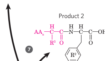
Enzyme-product 2 complex
