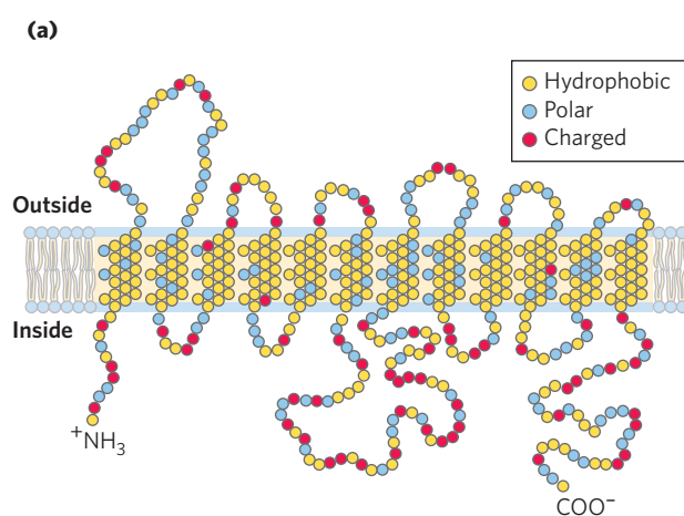
FIGURE 11-30 Membrane topology of the glucose transporter GLUT1. (a) Transmembrane helices are represented here as oblique (angled) rows of three or four amino acid residues, each row depicting one turn of the \alpha helix. Nine of the 12 helices contain three or more polar or charged residues (blue or red), often separated by several hydrophobic residues (yellow). This representation of topology is not intended to depict three-dimensional structure. (b) A helical wheel diagram shows the distribution of polar and nonpolar residues on the surface of a helical segment. The helix is diagrammed as though observed along its axis from the amino terminus. Adjacent residues in the linear sequence are
