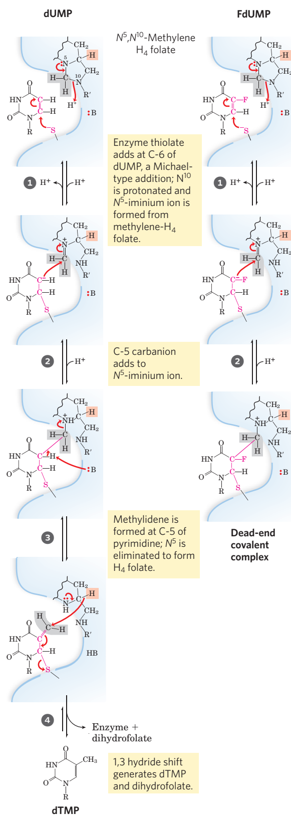
The 1,3 hydride shift (step ④), moves a hydride ion (shaded light red) from C-6 of H_4 folate to the methyl group of thymidine, resulting in the oxidation of tetrahydrofolate to dihydrofolate. This hydride shift is blocked when FdUMP is the substrate (right). Steps ① and ② proceed normally, but result in a stable complex—consisting of FdUMP linked covalently to the enzyme and to tetrahydrofolate—that inactivates the enzyme. Thymidylate Synthase Mechanism
