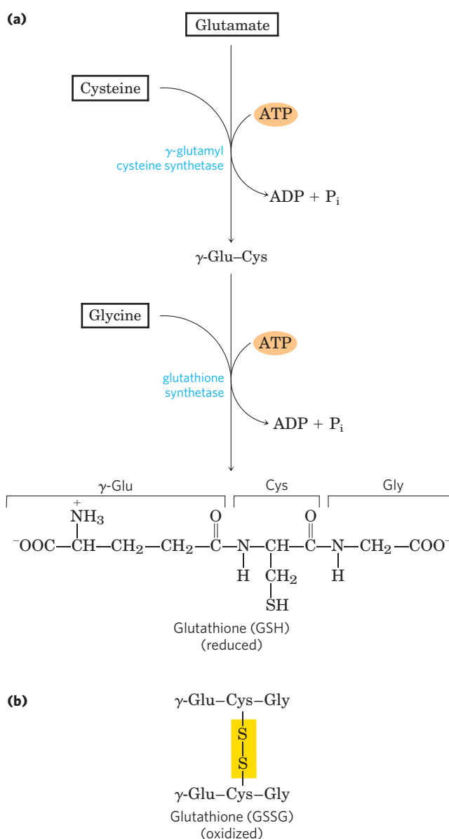
FIGURE 22-29 Glutathione metabolism. (a) Biosynthesis of glutathione. (b) Oxidized form of glutathione.
