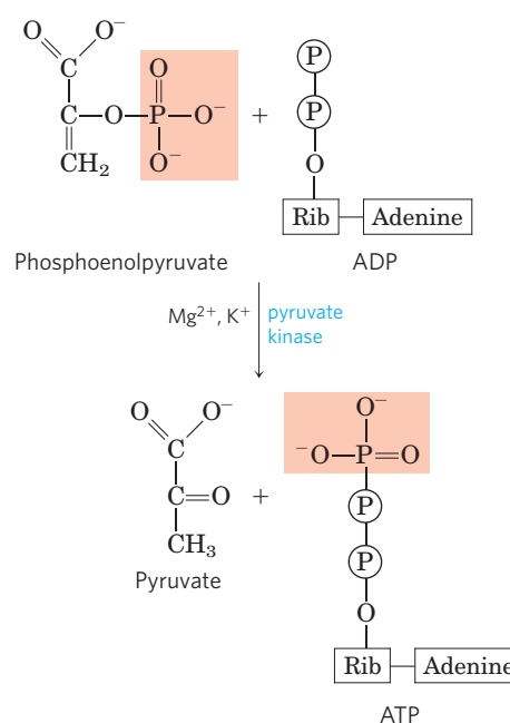
\Delta G'^{\circ} = -31.4 \text{ kJ/mol}
