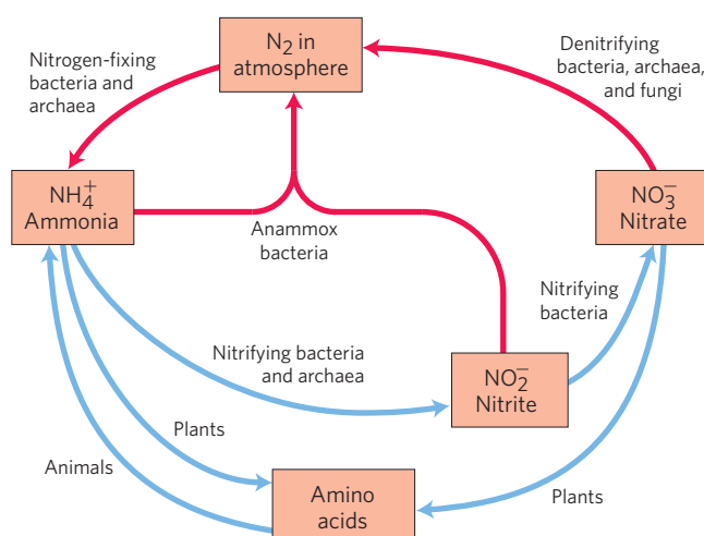
FIGURE 2 Cycling of nitrogen in the biosphere. Gaseous nitrogen ( N_2 ) makes up 80% of the earth's atmosphere.
