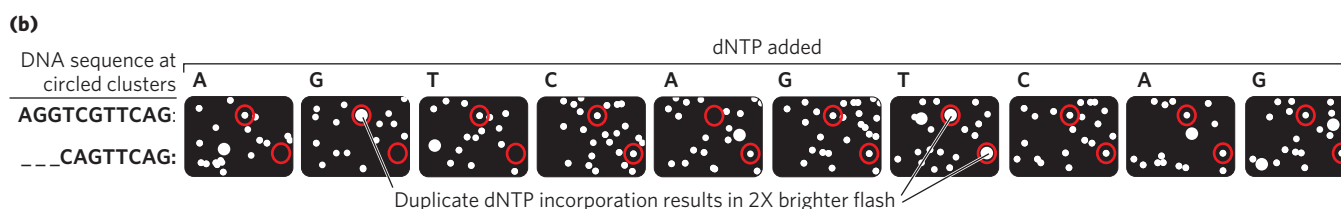
FIGURE 9-25 Next-generation pyrosequencing. (a) Pyrosequencing uses the enzymes sulfurylase (see Fig. 22-15) and luciferase (see Box 13-1) to detect nucleotide addition with flashes of light. The plot shows the light intensities observed during successive sequencing cycles for a DNA segment immobilized at a particular spot of a picotiter plate and (at top) the DNA nucleotide sequence derived from them. (b) An image of a very small part of one cycle of a 454 sequencing run. Each individual segment of DNA to be sequenced is attached to a tiny DNA capture bead, then amplified on the bead by PCR. Each bead is immersed in an emulsion and placed in a tiny (~29 μm) well on a picotiter plate. The reaction of luciferin and ATP with luciferase produces light flashes when a nucleotide is added to a particular DNA cluster in a particular well. Circles represent the same cluster over multiple cycles. In this case, reading the top (or bottom) circle from left to right across each row gives the sequence for that cluster.
