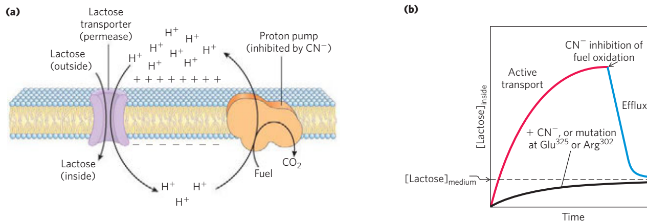
FIGURE 11-41 Lactose uptake in E. coli . (a) The primary transport of \text{H}^+ out of the cell, driven by the oxidation of a variety of fuels, establishes both a proton gradient and an electrical potential (inside negative) across the membrane. Secondary active transport of lactose into the cell involves symport of \text{H}^+ and lactose by the lactose transporter. The uptake of lactose against its concentration gradient is entirely dependent on this inflow
