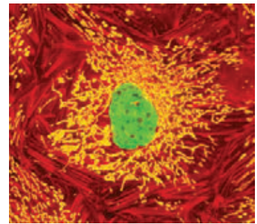
FIGURE 19-42 Single cells contain many mitochondria. A typical animal cell has hundreds or thousands of mitochondria, some fraction of which may contain genomes with mutations that affect mitochondrial function. This ovine (sheep) kidney epithelial cell was cultured in the laboratory, fixed, and then stained with fluorescent probes that show mitochondria as gold, microfilaments of actin as red, and nuclei as green when observed in the fluorescence microscope.
