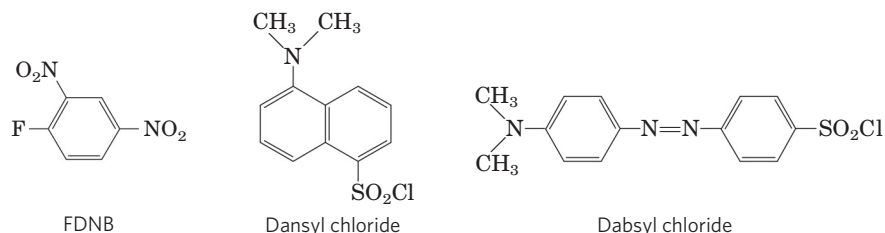
FIGURE 3-26 Reagents used to modify the \alpha -amino group at the amino terminus.
